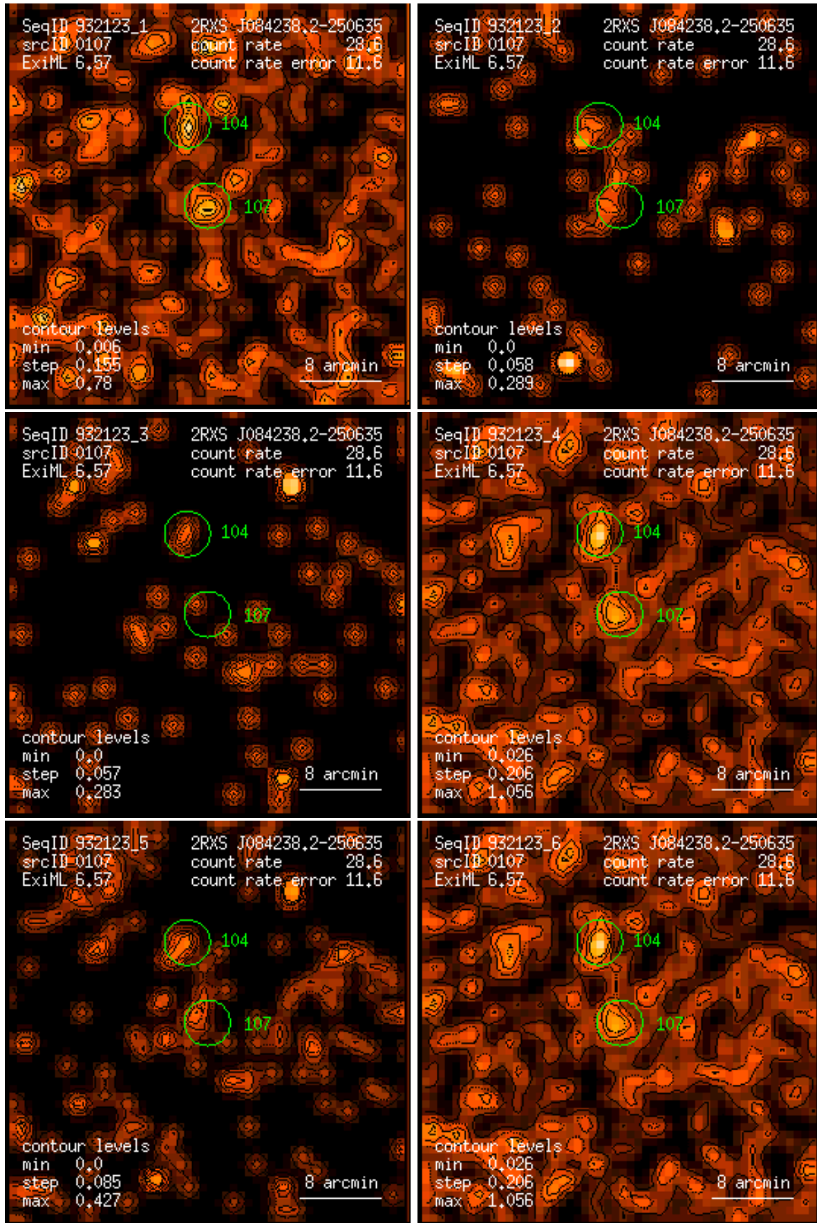
Figure 107: RASS 932123: detection 0107: band rate images, Gaussian filter: (1) PSPC channels 11 – 41, (2) 52 – 90, (3) 91 – 201, (4) 11 – 235, (5) 52 – 201, (6) 11 – 201. Broad band rates in counts/ks. Band rate contour levels in counts/ks/arcmin 2 .
