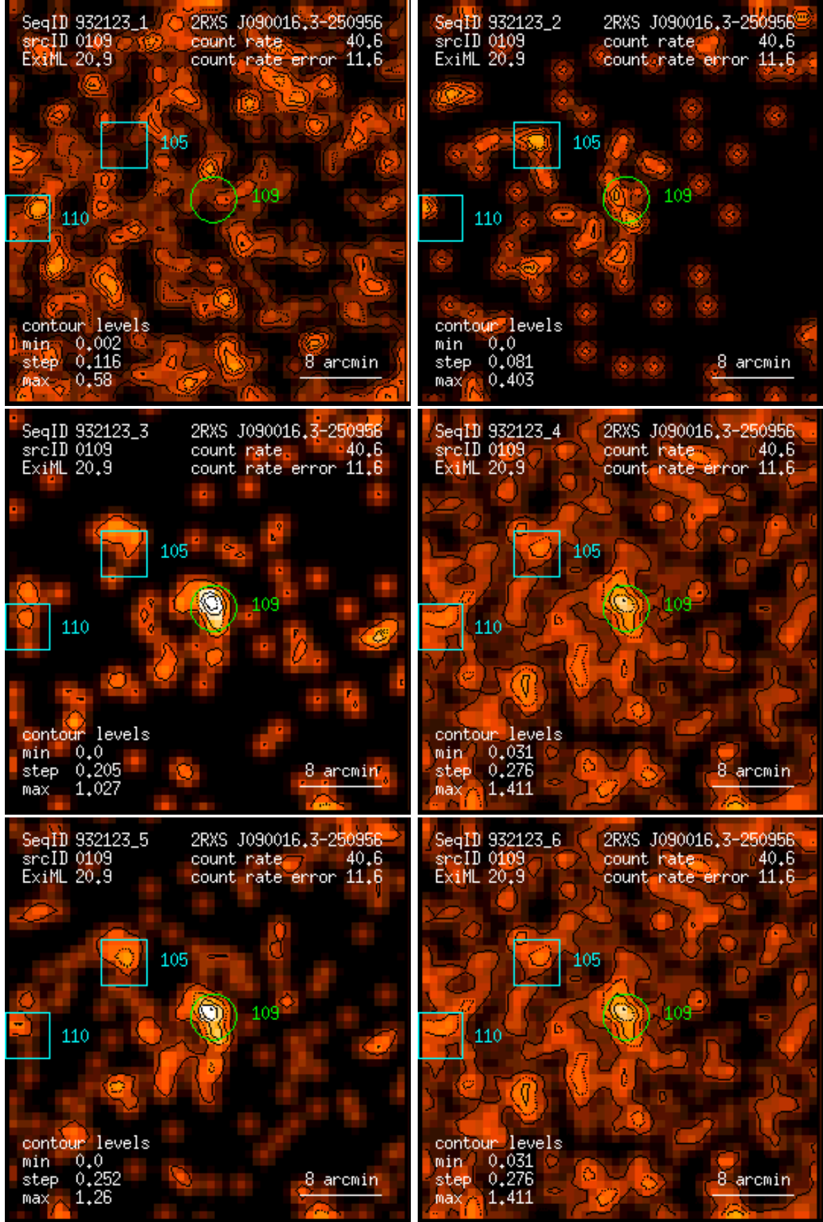
Figure 109: RASS 932123: detection 0109: band rate images, Gaussian filter: (1) PSPC channels 11 – 41, (2) 52 – 90, (3) 91 – 201, (4) 11 – 235, (5) 52 – 201, (6) 11 – 201. Broad band rates in counts/ks. Band rate contour levels in counts/ks/arcmin 2 .
