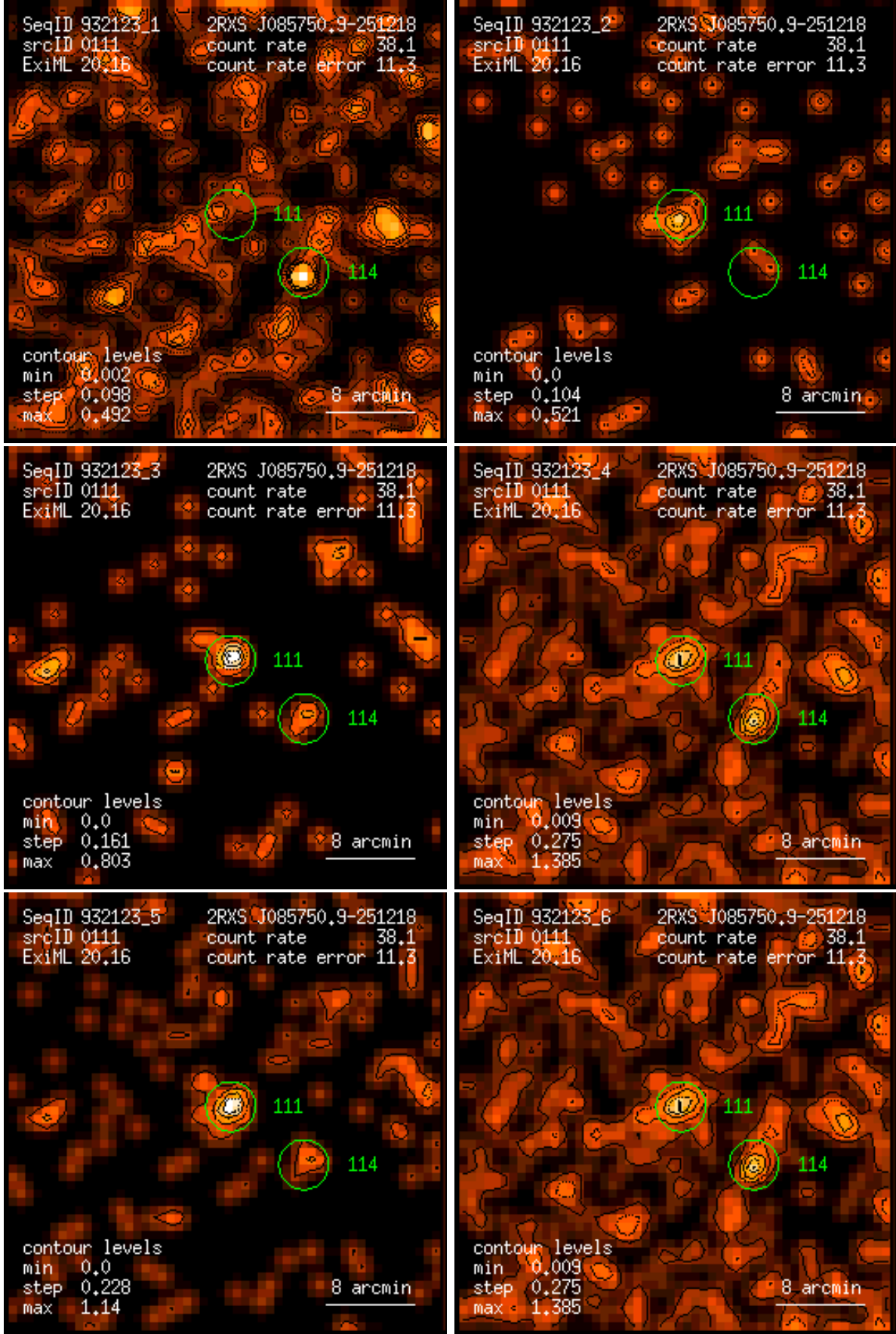
Figure 111: RASS 932123: detection 0111: band rate images, Gaussian filter: (1) PSPC channels 11 – 41, (2) 52 – 90, (3) 91 – 201, (4) 11 – 235, (5) 52 – 201, (6) 11 – 201. Broad band rates in counts/ks. Band rate contour levels in counts/ks/arcmin 2 .
