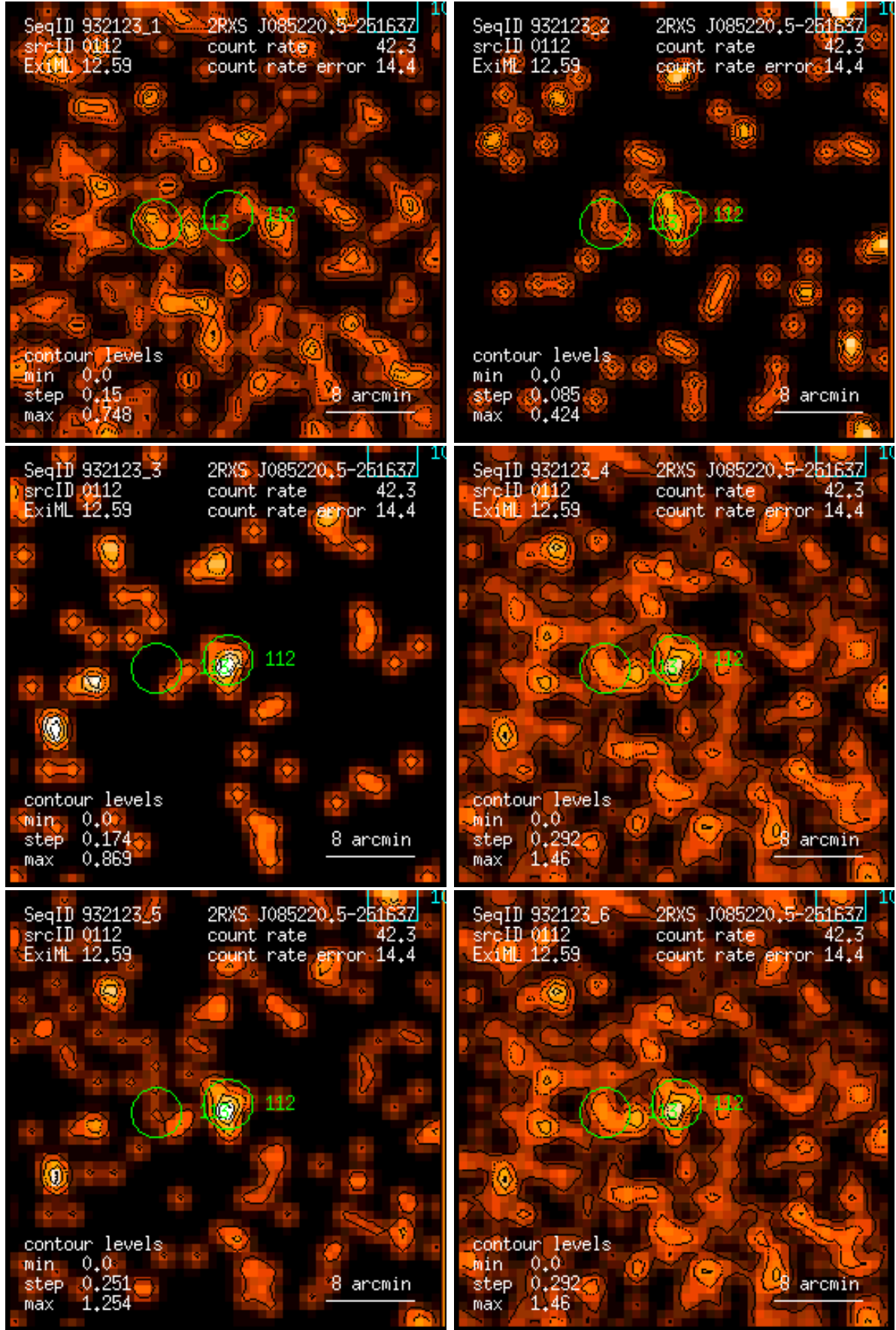
Figure 112: RASS 932123: detection 0112: band rate images, Gaussian filter: (1) PSPC channels 11 – 41, (2) 52 – 90, (3) 91 – 201, (4) 11 – 235, (5) 52 – 201, (6) 11 – 201. Broad band rates in counts/ks. Band rate contour levels in counts/ks/arcmin 2 .
