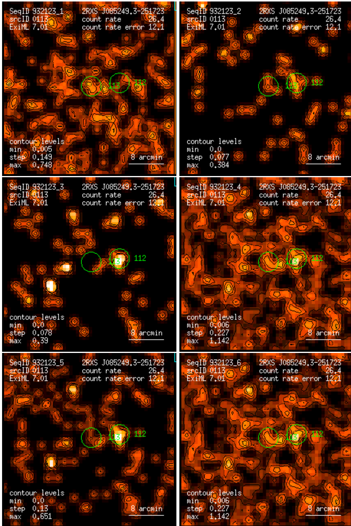
Figure 113: RASS 932123: detection 0113: band rate images, Gaussian filter: (1) PSPC channels 11 – 41, (2) 52 – 90, (3) 91 – 201, (4) 11 – 235, (5) 52 – 201, (6) 11 – 201. Broad band rates in counts/ks. Band rate contour levels in counts/ks/arcmin 2 .
