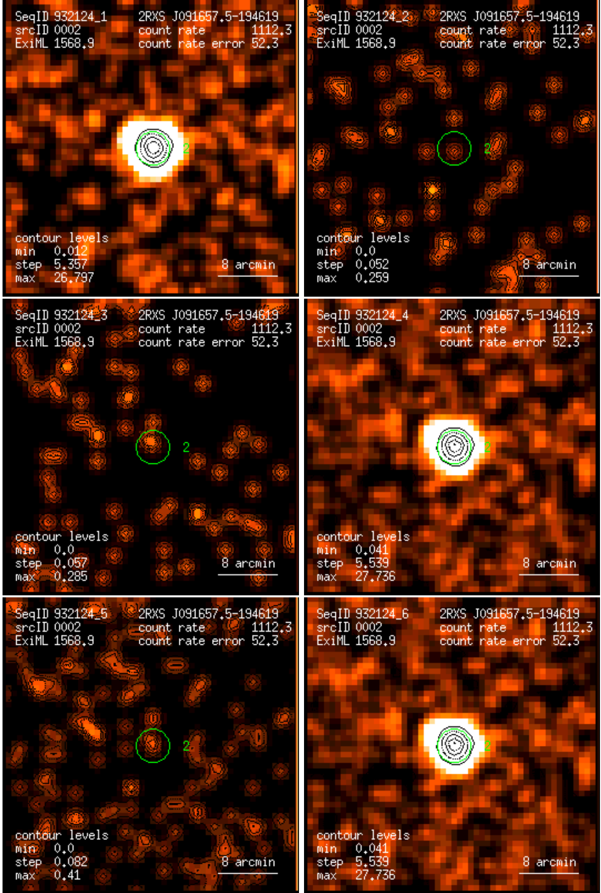
Figure 2: RASS 932124: detection 0002: band rate images, Gaussian filter: (1) PSPC channels 11 – 41, (2) 52 – 90, (3) 91 – 201, (4) 11 – 235, (5) 52 – 201, (6) 11 – 201. Broad band rates in counts/ks. Band rate contour levels in counts/ks/arcmin 2 .
