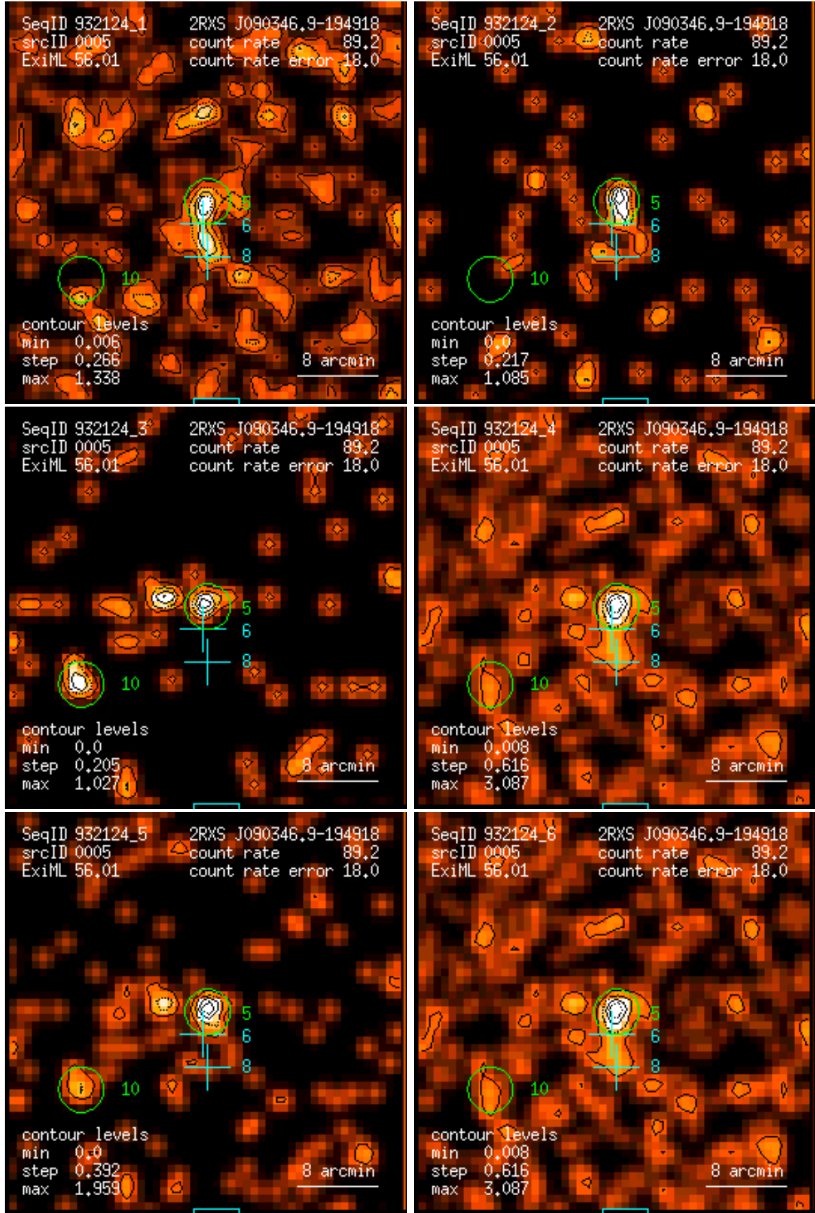
Figure 5: RASS 932124: detection 0005: band rate images, Gaussian filter: (1) PSPC channels 11 – 41, (2) 52 – 90, (3) 91 – 201, (4) 11 – 235, (5) 52 – 201, (6) 11 – 201. Broad band rates in counts/ks. Band rate contour levels in counts/ks/arcmin 2 .
