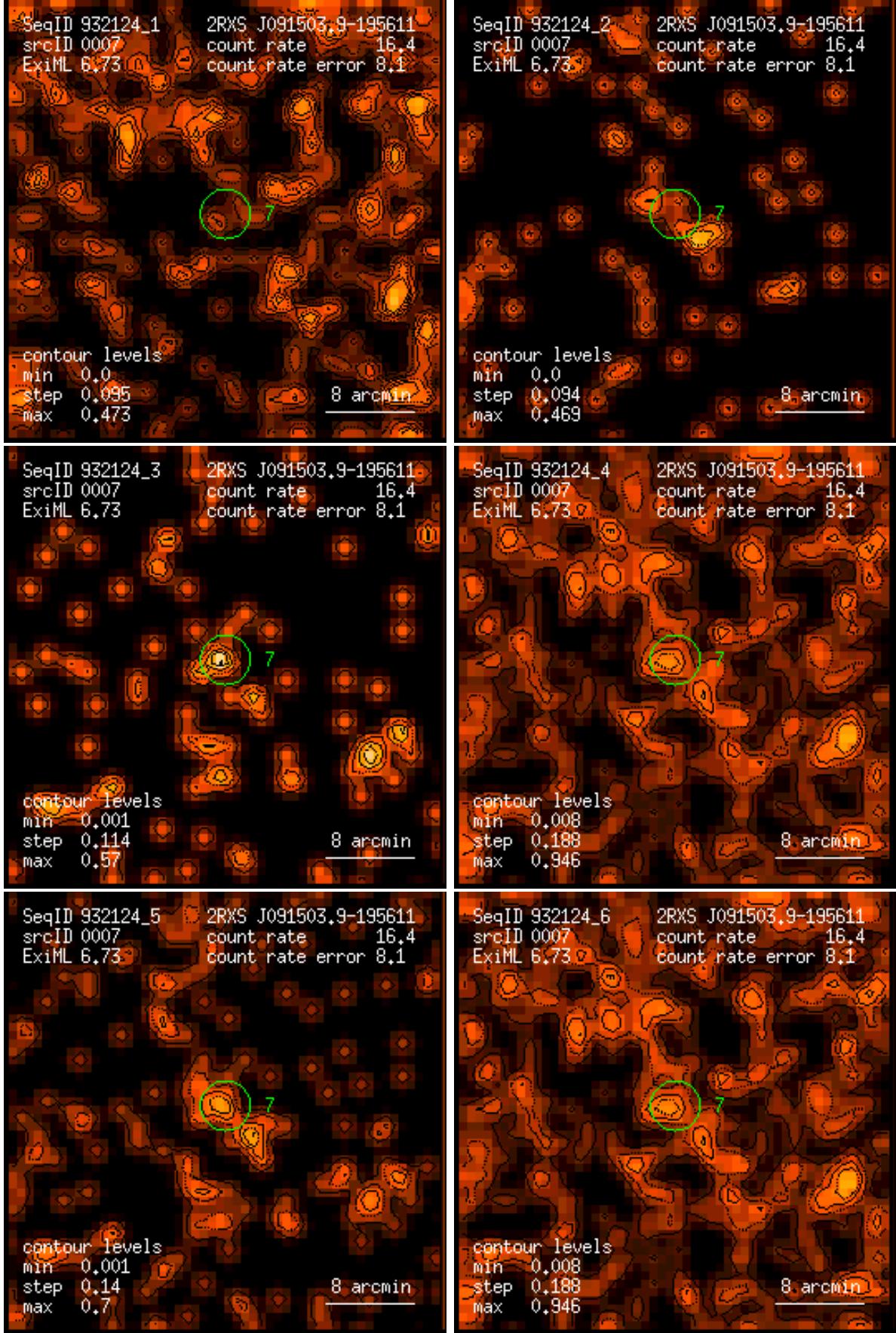
Figure 7: RASS 932124: detection 0007: band rate images, Gaussian filter: (1) PSPC channels 11 – 41, (2) 52 – 90, (3) 91 – 201, (4) 11 – 235, (5) 52 – 201, (6) 11 – 201. Broad band rates in counts/ks. Band rate contour levels in counts/ks/arcmin 2 .
