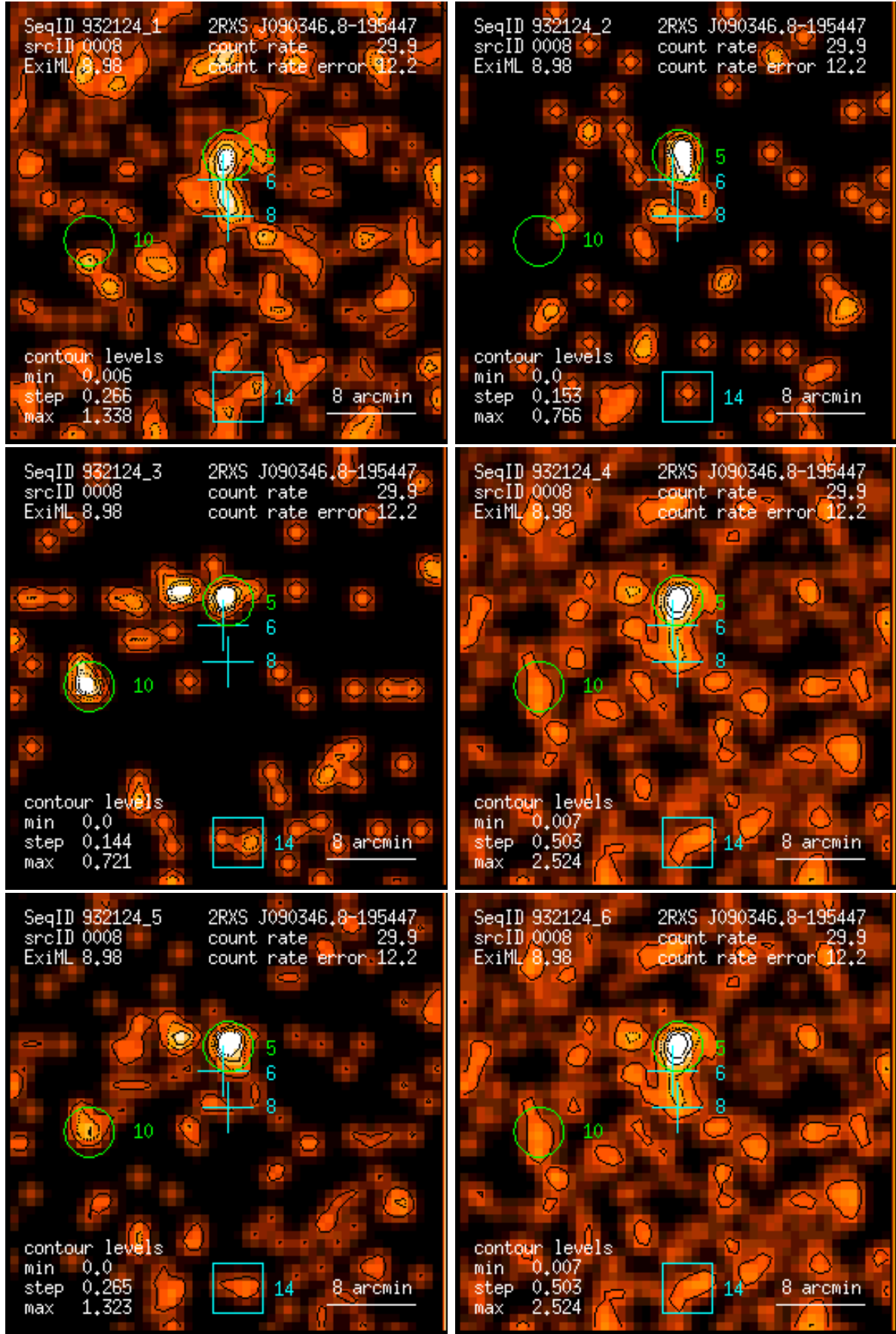
Figure 8: RASS 932124: detection 0008: band rate images, Gaussian filter: (1) PSPC channels 11 – 41, (2) 52 – 90, (3) 91 – 201, (4) 11 – 235, (5) 52 – 201, (6) 11 – 201. Broad band rates in counts/ks. Band rate contour levels in counts/ks/arcmin 2 .
