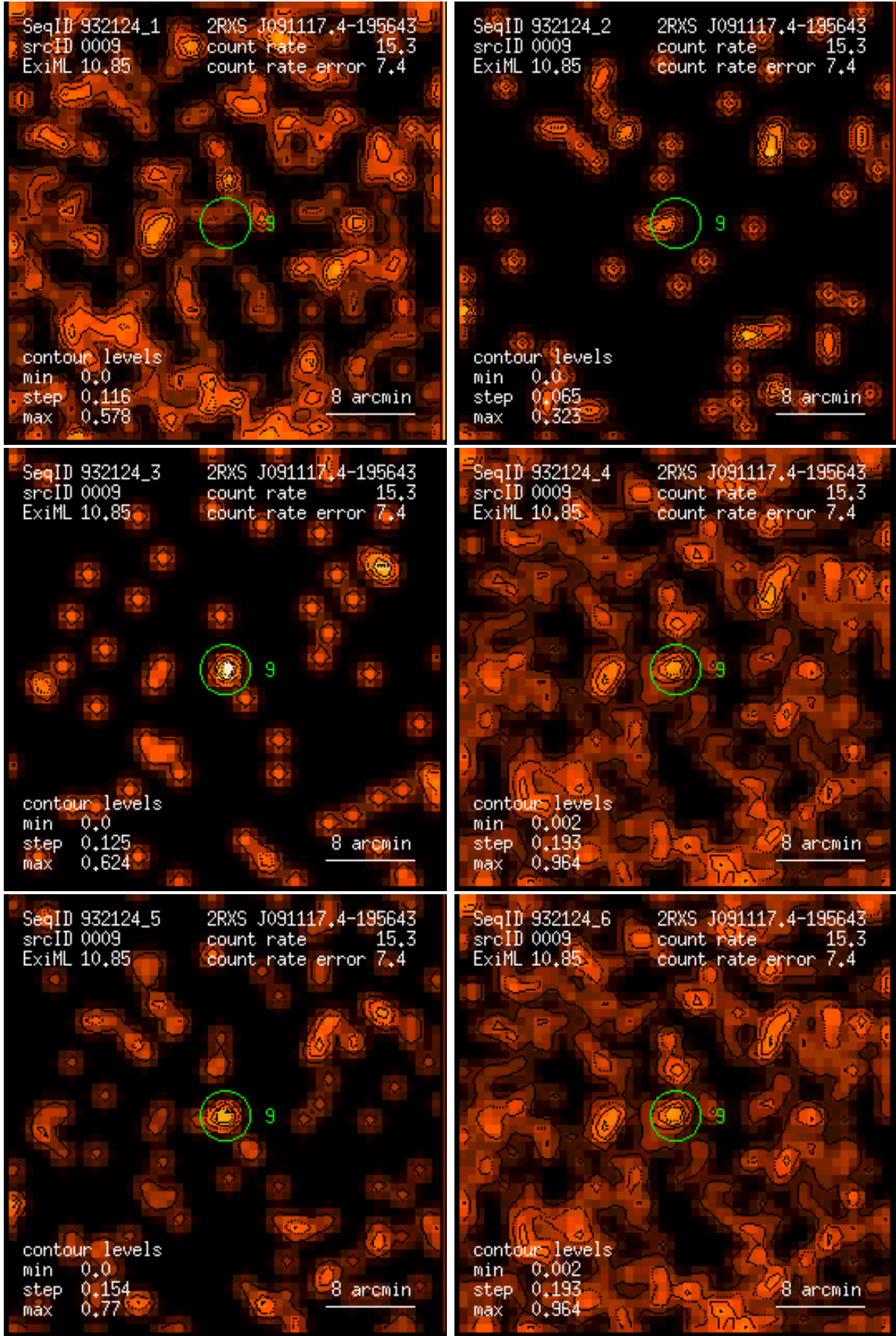
Figure 9: RASS 932124: detection 0009: band rate images, Gaussian filter: (1) PSPC channels 11 – 41, (2) 52 – 90, (3) 91 – 201, (4) 11 – 235, (5) 52 – 201, (6) 11 – 201. Broad band rates in counts/ks. Band rate contour levels in counts/ks/arcmin 2 .
