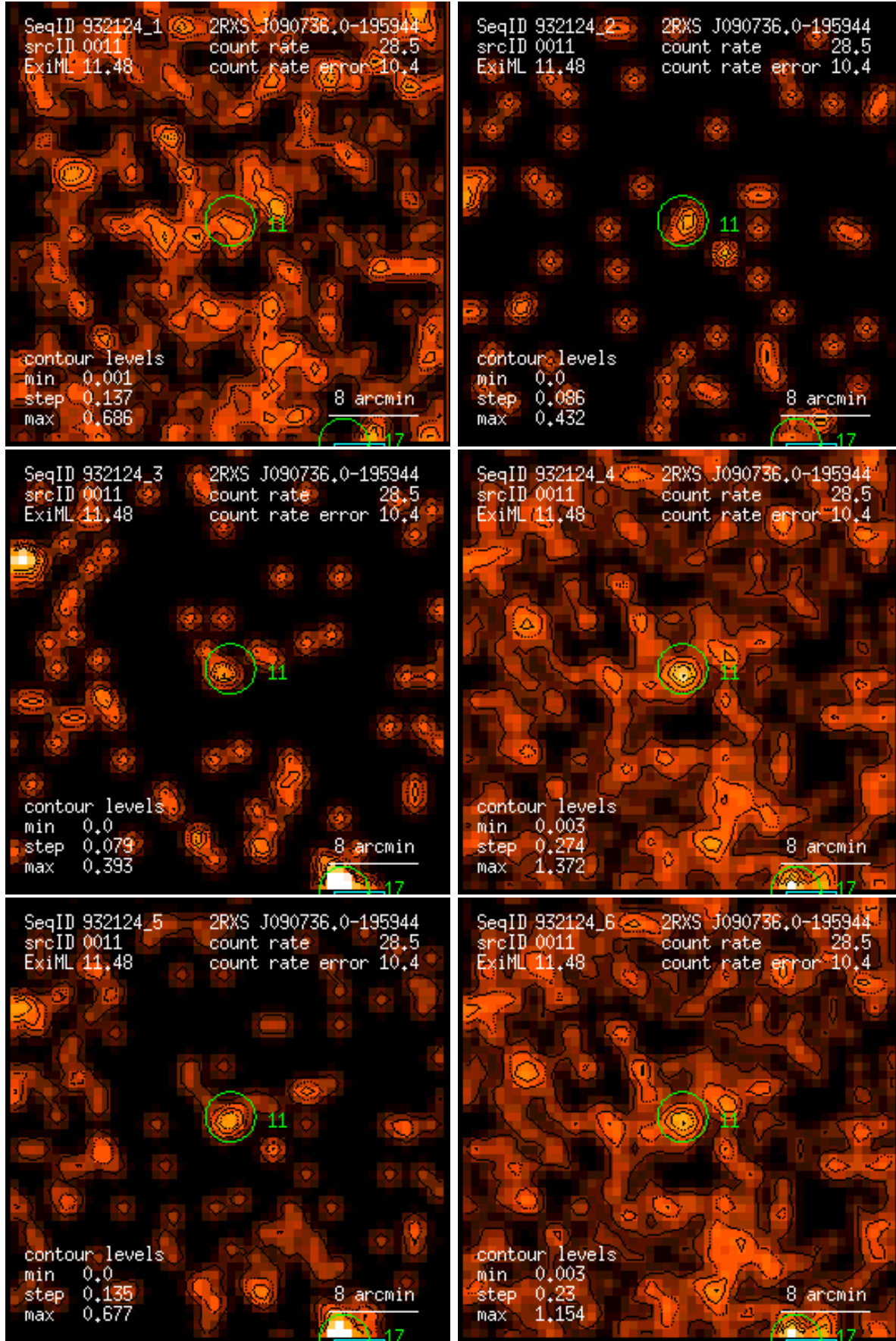
Figure 11: RASS 932124: detection 0011: band rate images, Gaussian filter: (1) PSPC channels 11 – 41, (2) 52 – 90, (3) 91 – 201, (4) 11 – 235, (5) 52 – 201, (6) 11 – 201. Broad band rates in counts/ks. Band rate contour levels in counts/ks/arcmin 2 .
