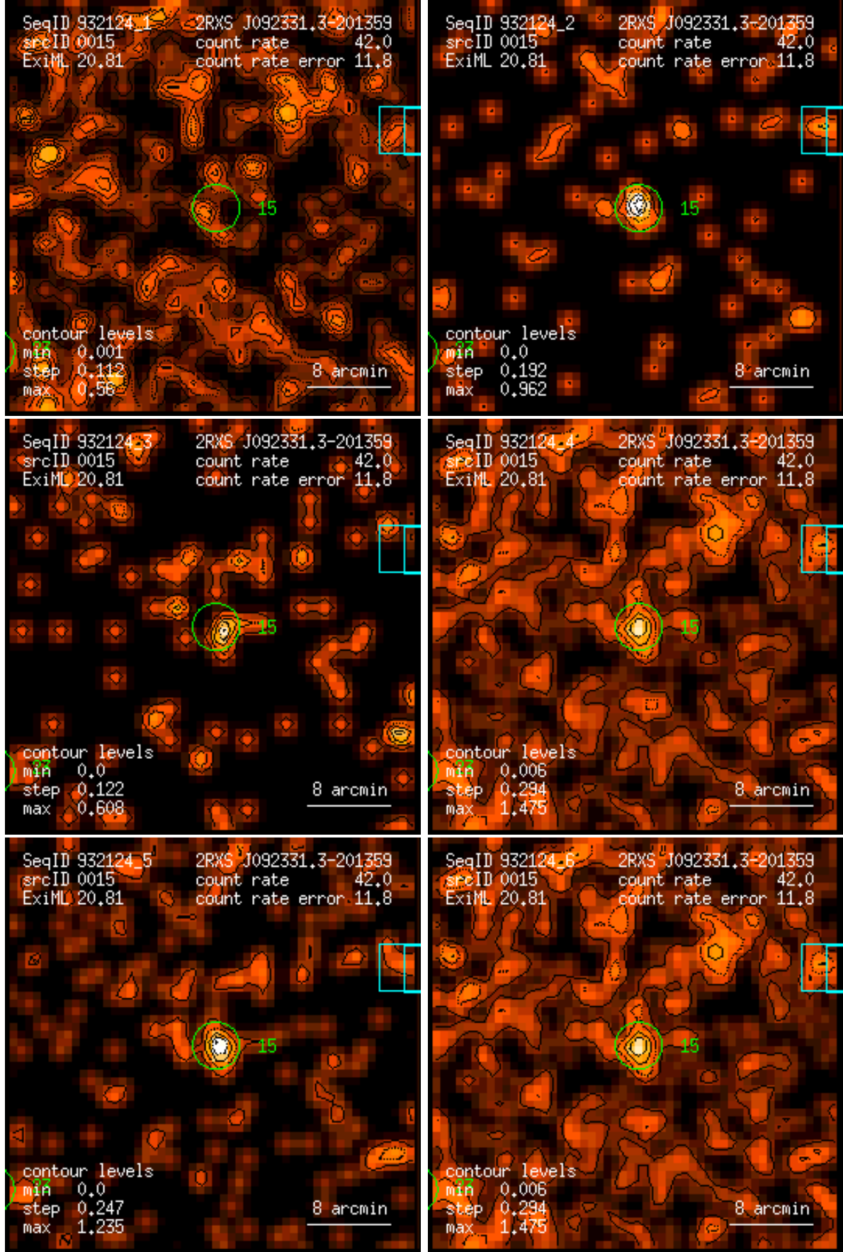
Figure 15: RASS 932124: detection 0015: band rate images, Gaussian filter: (1) PSPC channels 11 – 41, (2) 52 – 90, (3) 91 – 201, (4) 11 – 235, (5) 52 – 201, (6) 11 – 201. Broad band rates in counts/ks. Band rate contour levels in counts/ks/arcmin 2 .
