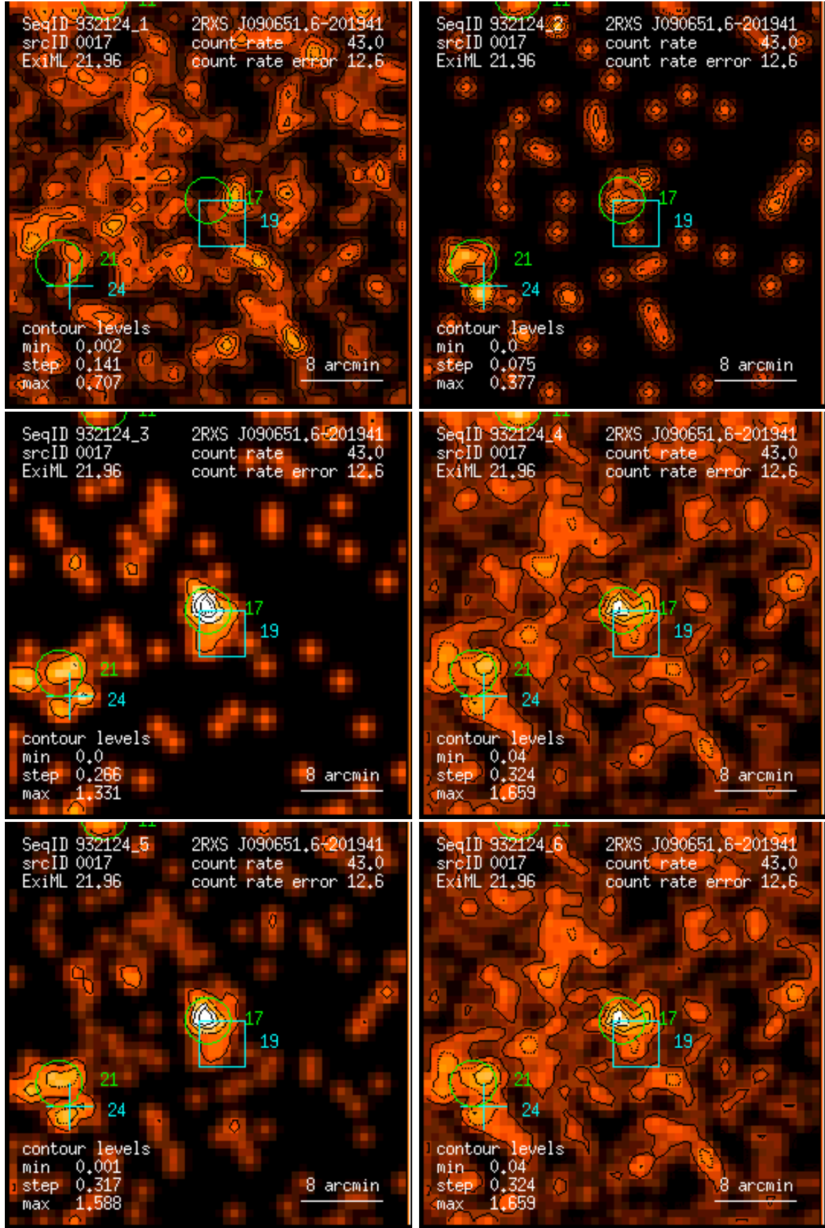
Figure 17: RASS 932124: detection 0017: band rate images, Gaussian filter: (1) PSPC channels 11 – 41, (2) 52 – 90, (3) 91 – 201, (4) 11 – 235, (5) 52 – 201, (6) 11 – 201. Broad band rates in counts/ks. Band rate contour levels in counts/ks/arcmin 2 .
