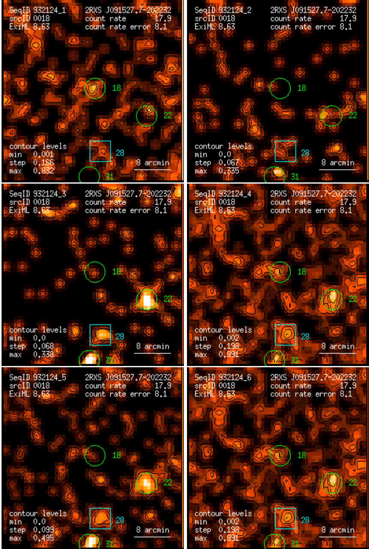
Figure 18: RASS 932124: detection 0018: band rate images, Gaussian filter: (1) PSPC channels 11 – 41, (2) 52 – 90, (3) 91 – 201, (4) 11 – 235, (5) 52 – 201, (6) 11 – 201. Broad band rates in counts/ks. Band rate contour levels in counts/ks/arcmin 2 .
