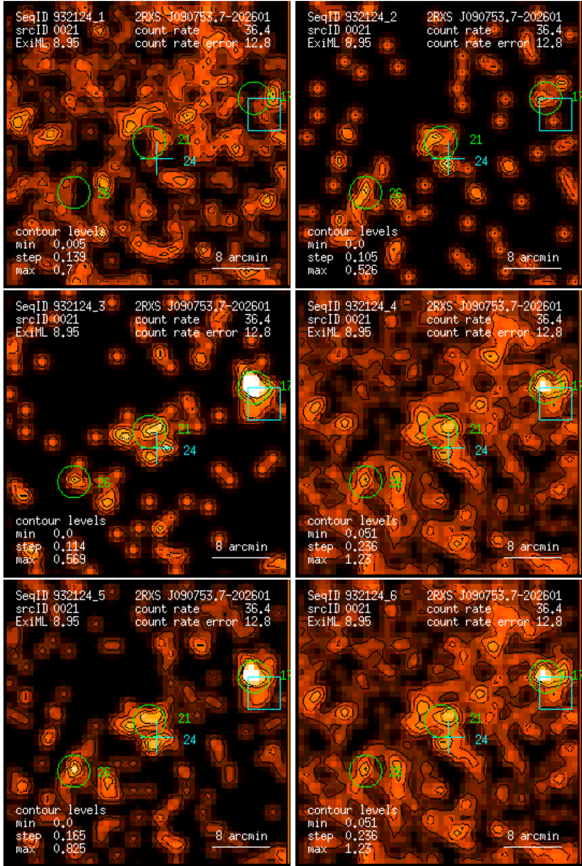
Figure 21: RASS 932124: detection 0021: band rate images, Gaussian filter: (1) PSPC channels 11 – 41, (2) 52 – 90, (3) 91 – 201, (4) 11 – 235, (5) 52 – 201, (6) 11 – 201. Broad band rates in counts/ks. Band rate contour levels in counts/ks/arcmin 2 .
