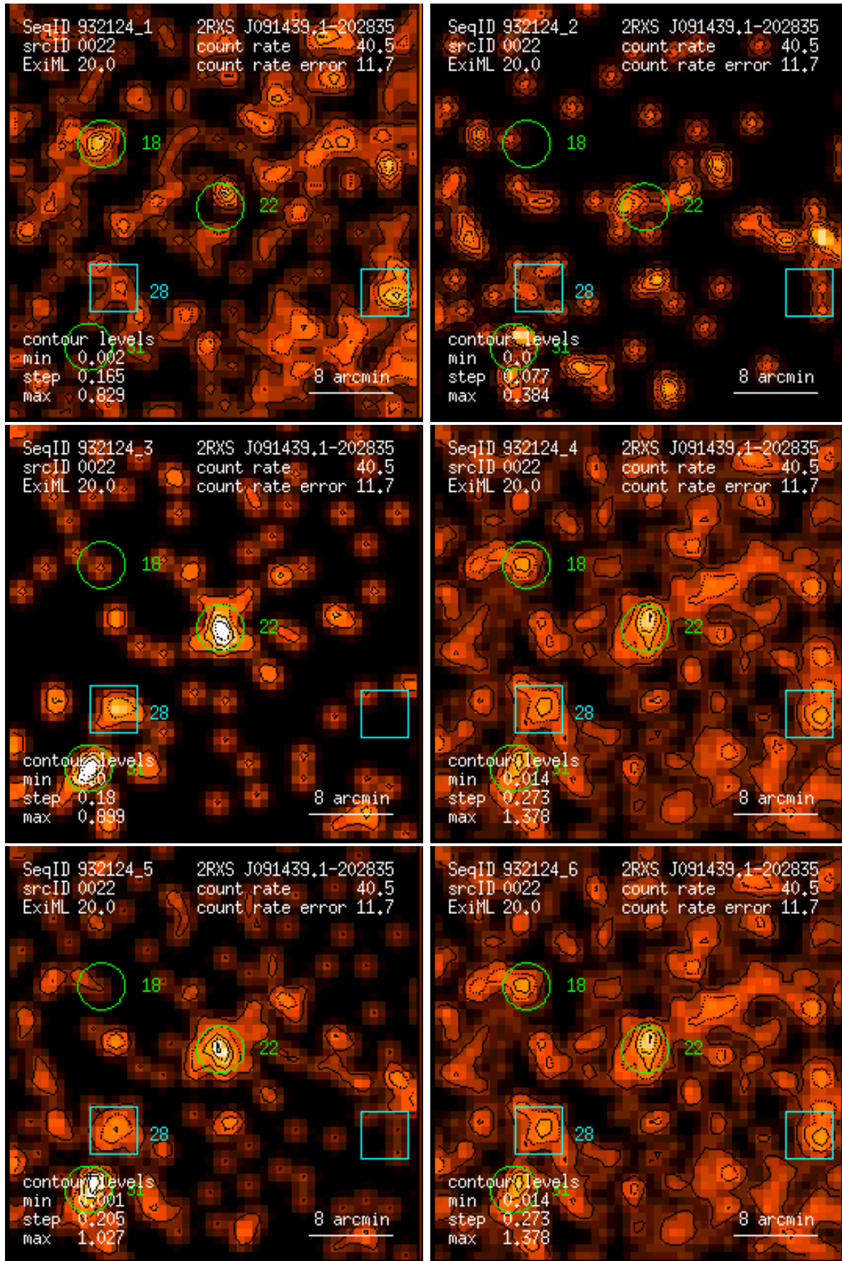
Figure 22: RASS 932124: detection 0022: band rate images, Gaussian filter: (1) PSPC channels 11 – 41, (2) 52 – 90, (3) 91 – 201, (4) 11 – 235, (5) 52 – 201, (6) 11 – 201. Broad band rates in counts/ks. Band rate contour levels in counts/ks/arcmin 2 .
