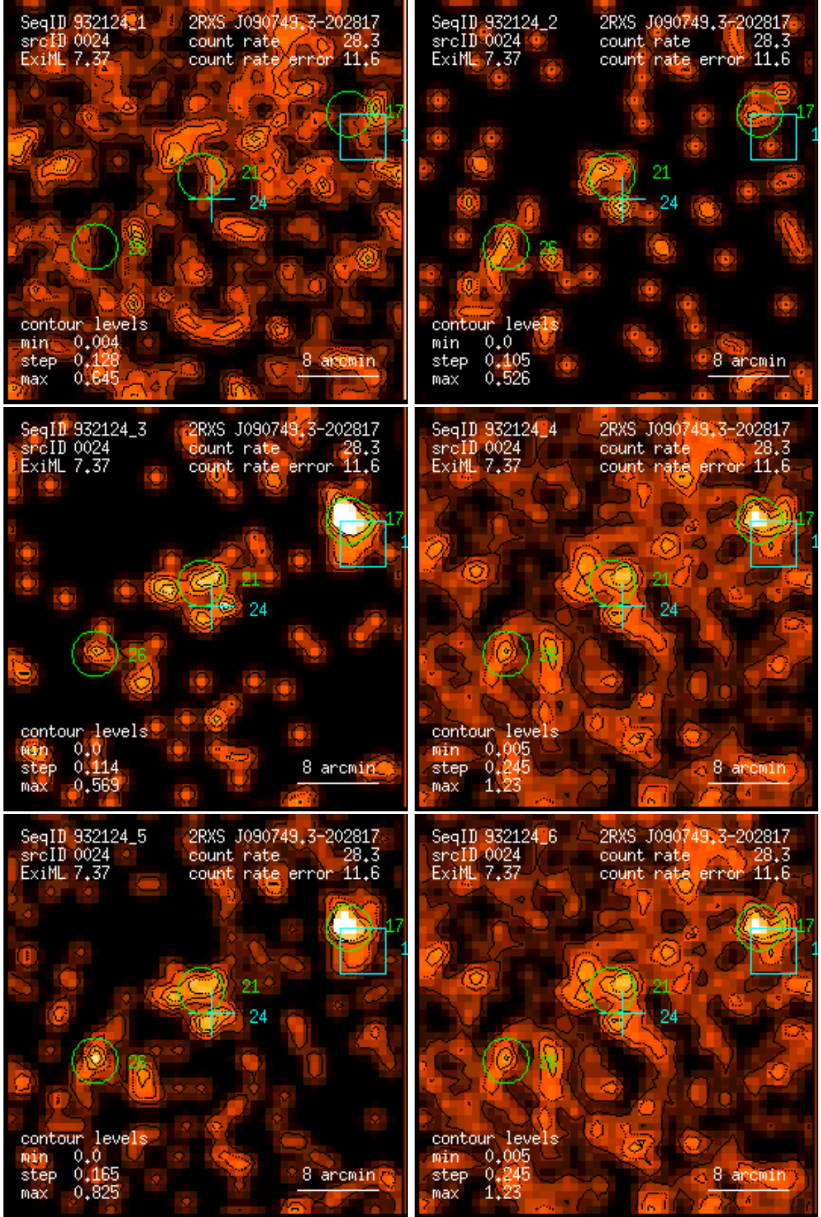
Figure 24: RASS 932124: detection 0024: band rate images, Gaussian filter: (1) PSPC channels 11 – 41, (2) 52 – 90, (3) 91 – 201, (4) 11 – 235, (5) 52 – 201, (6) 11 – 201. Broad band rates in counts/ks. Band rate contour levels in counts/ks/arcmin 2 .
