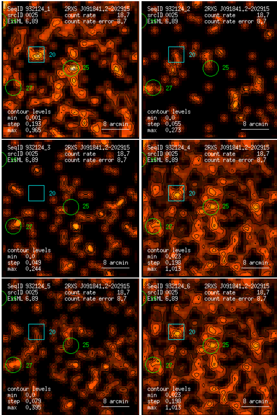
Figure 25: RASS 932124: detection 0025: band rate images, Gaussian filter: (1) PSPC channels 11 – 41, (2) 52 – 90, (3) 91 – 201, (4) 11 – 235, (5) 52 – 201, (6) 11 – 201. Broad band rates in counts/ks. Band rate contour levels in counts/ks/arcmin 2 .
