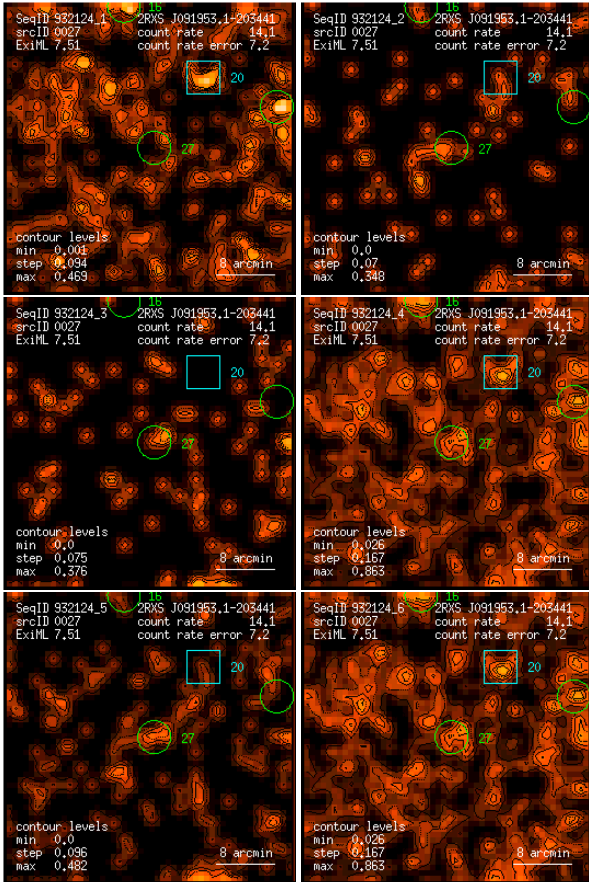
Figure 27: RASS 932124: detection 0027: band rate images, Gaussian filter: (1) PSPC channels 11 – 41, (2) 52 – 90, (3) 91 – 201, (4) 11 – 235, (5) 52 – 201, (6) 11 – 201. Broad band rates in counts/ks. Band rate contour levels in counts/ks/arcmin 2 .
