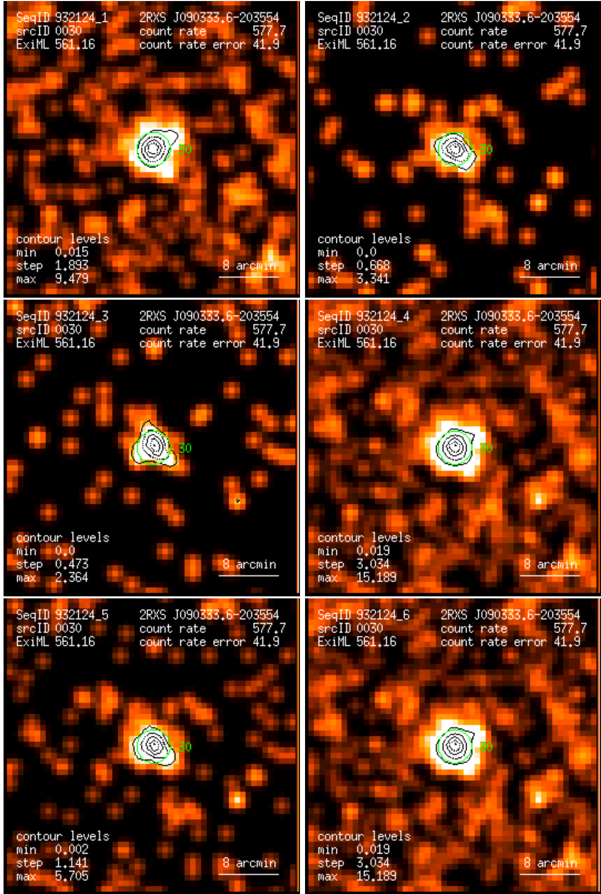
Figure 30: RASS 932124: detection 0030: band rate images, Gaussian filter: (1) PSPC channels 11 – 41, (2) 52 – 90, (3) 91 – 201, (4) 11 – 235, (5) 52 – 201, (6) 11 – 201. Broad band rates in counts/ks. Band rate contour levels in counts/ks/arcmin 2 .
