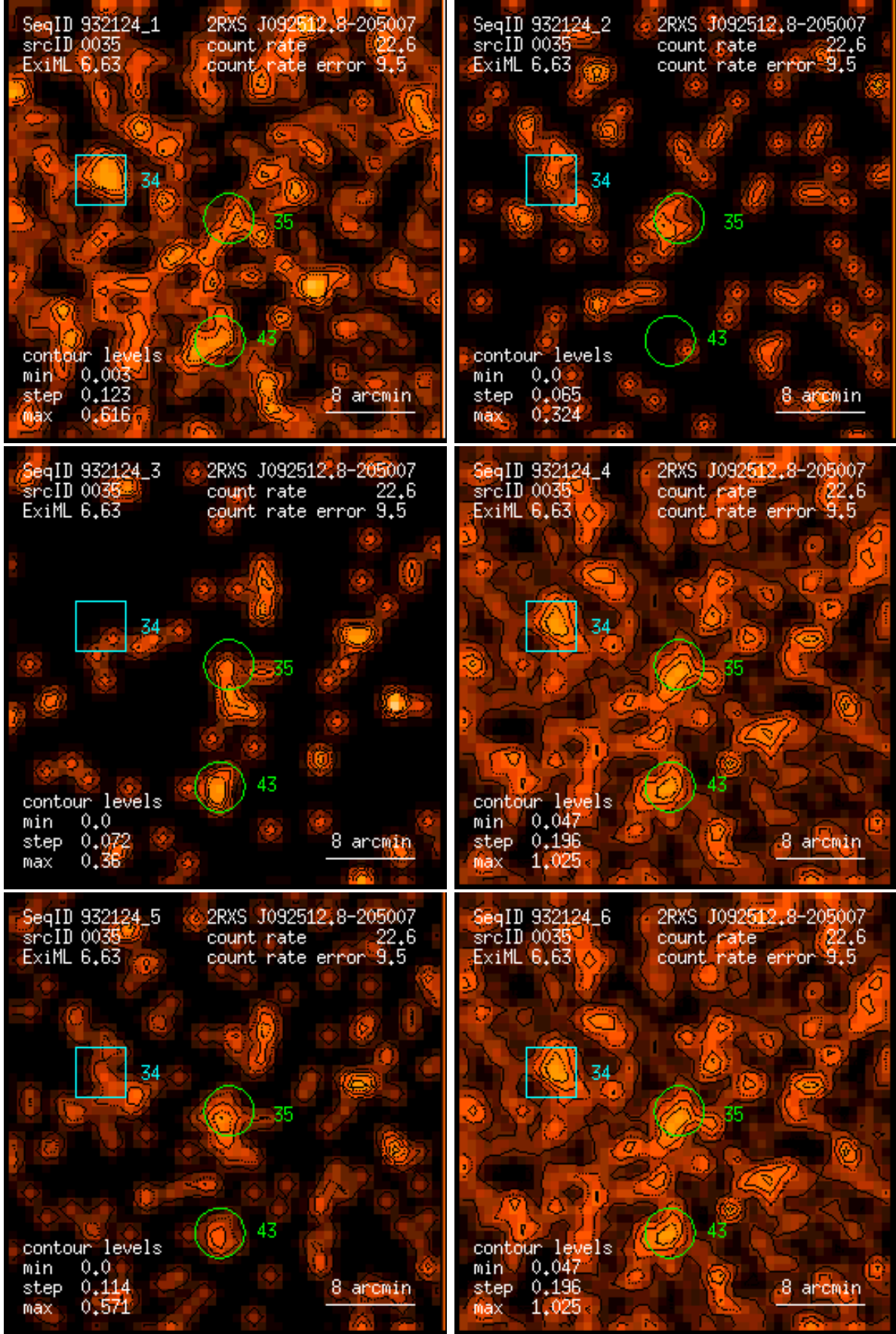
Figure 35: RASS 932124: detection 0035: band rate images, Gaussian filter: (1) PSPC channels 11 – 41, (2) 52 – 90, (3) 91 – 201, (4) 11 – 235, (5) 52 – 201, (6) 11 – 201. Broad band rates in counts/ks. Band rate contour levels in counts/ks/arcmin 2 .
