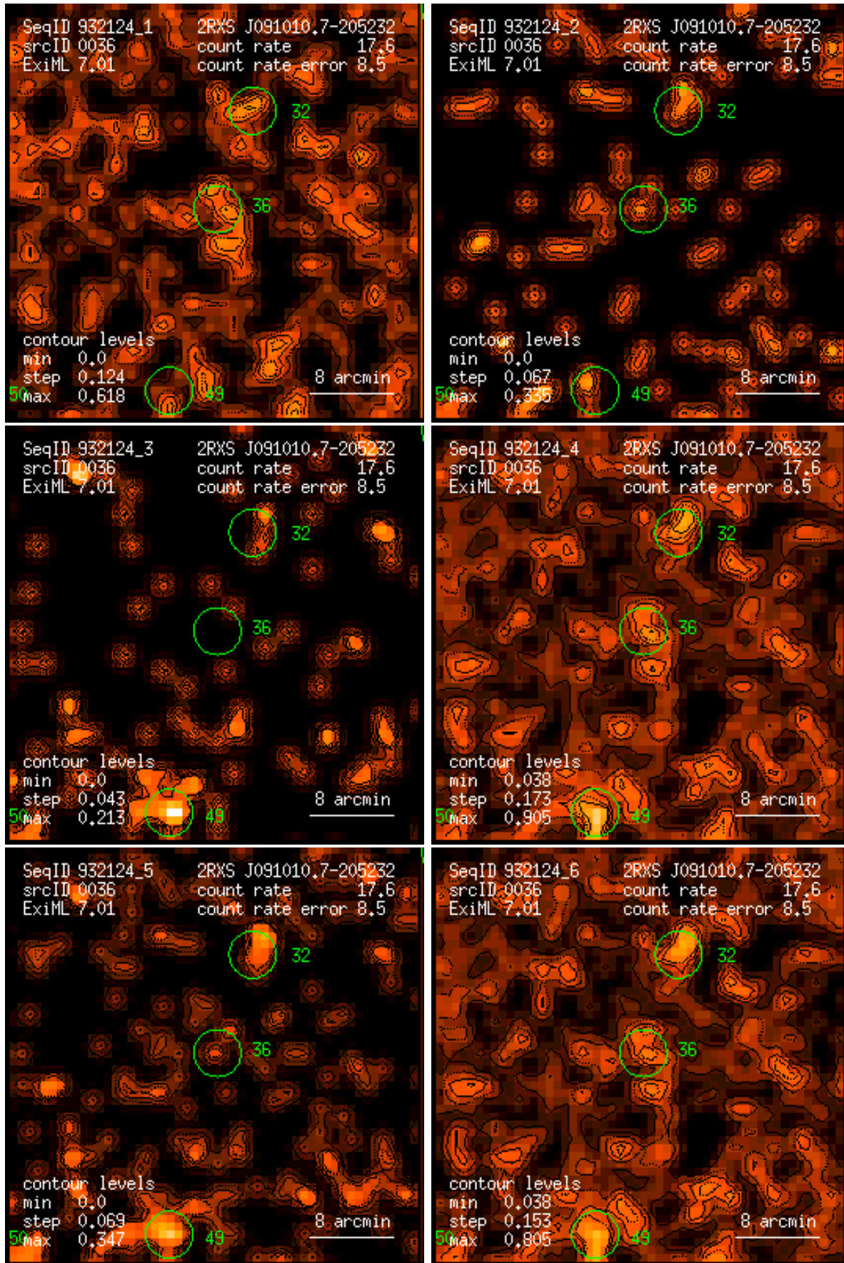
Figure 36: RASS 932124: detection 0036: band rate images, Gaussian filter: (1) PSPC channels 11 – 41, (2) 52 – 90, (3) 91 – 201, (4) 11 – 235, (5) 52 – 201, (6) 11 – 201. Broad band rates in counts/ks. Band rate contour levels in counts/ks/arcmin 2 .
