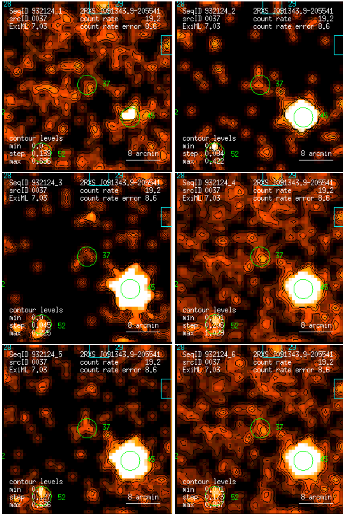
Figure 37: RASS 932124: detection 0037: band rate images, Gaussian filter: (1) PSPC channels 11 – 41, (2) 52 – 90, (3) 91 – 201, (4) 11 – 235, (5) 52 – 201, (6) 11 – 201. Broad band rates in counts/ks. Band rate contour levels in counts/ks/arcmin 2 .
