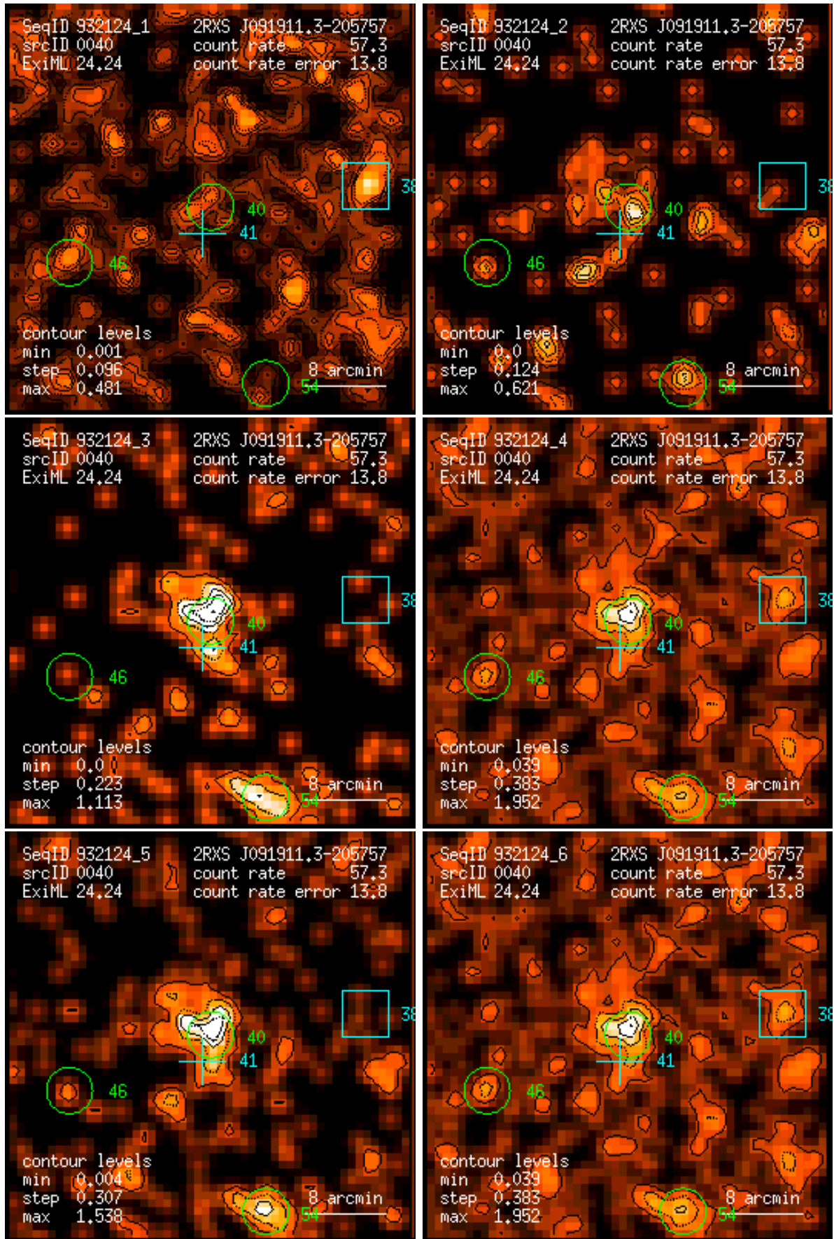
Figure 40: RASS 932124: detection 0040: band rate images, Gaussian filter: (1) PSPC channels 11 – 41, (2) 52 – 90, (3) 91 – 201, (4) 11 – 235, (5) 52 – 201, (6) 11 – 201. Broad band rates in counts/ks. Band rate contour levels in counts/ks/arcmin 2 .
