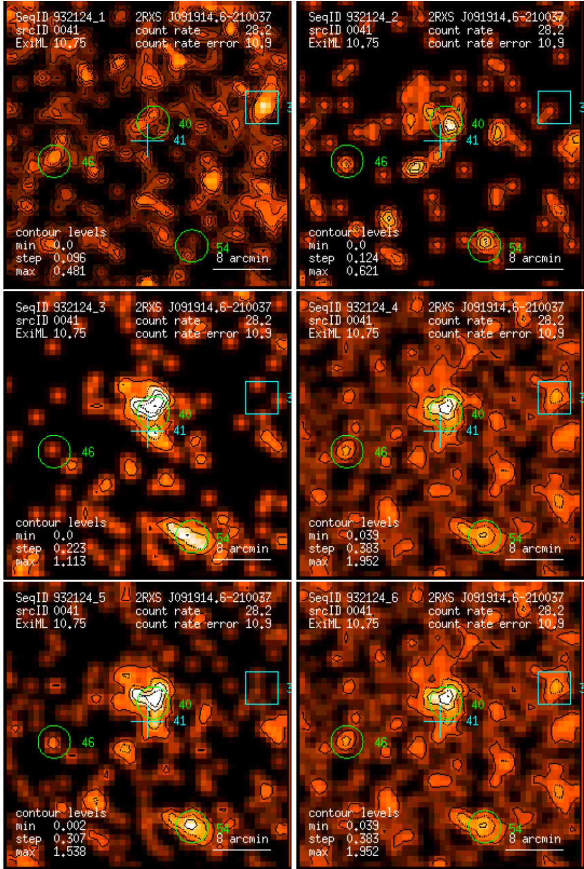
Figure 41: RASS 932124: detection 0041: band rate images, Gaussian filter: (1) PSPC channels 11 – 41, (2) 52 – 90, (3) 91 – 201, (4) 11 – 235, (5) 52 – 201, (6) 11 – 201. Broad band rates in counts/ks. Band rate contour levels in counts/ks/arcmin 2 .
