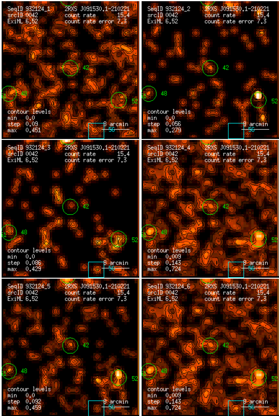
Figure 42: RASS 932124: detection 0042: band rate images, Gaussian filter: (1) PSPC channels 11 – 41, (2) 52 – 90, (3) 91 – 201, (4) 11 – 235, (5) 52 – 201, (6) 11 – 201. Broad band rates in counts/ks. Band rate contour levels in counts/ks/arcmin 2 .
