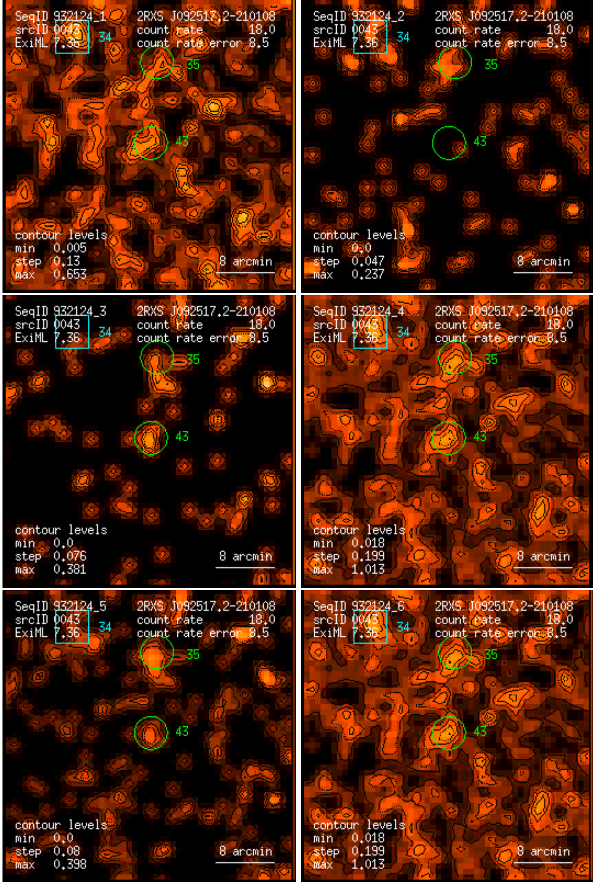
Figure 43: RASS 932124: detection 0043: band rate images, Gaussian filter: (1) PSPC channels 11 – 41, (2) 52 – 90, (3) 91 – 201, (4) 11 – 235, (5) 52 – 201, (6) 11 – 201. Broad band rates in counts/ks. Band rate contour levels in counts/ks/arcmin 2 .
