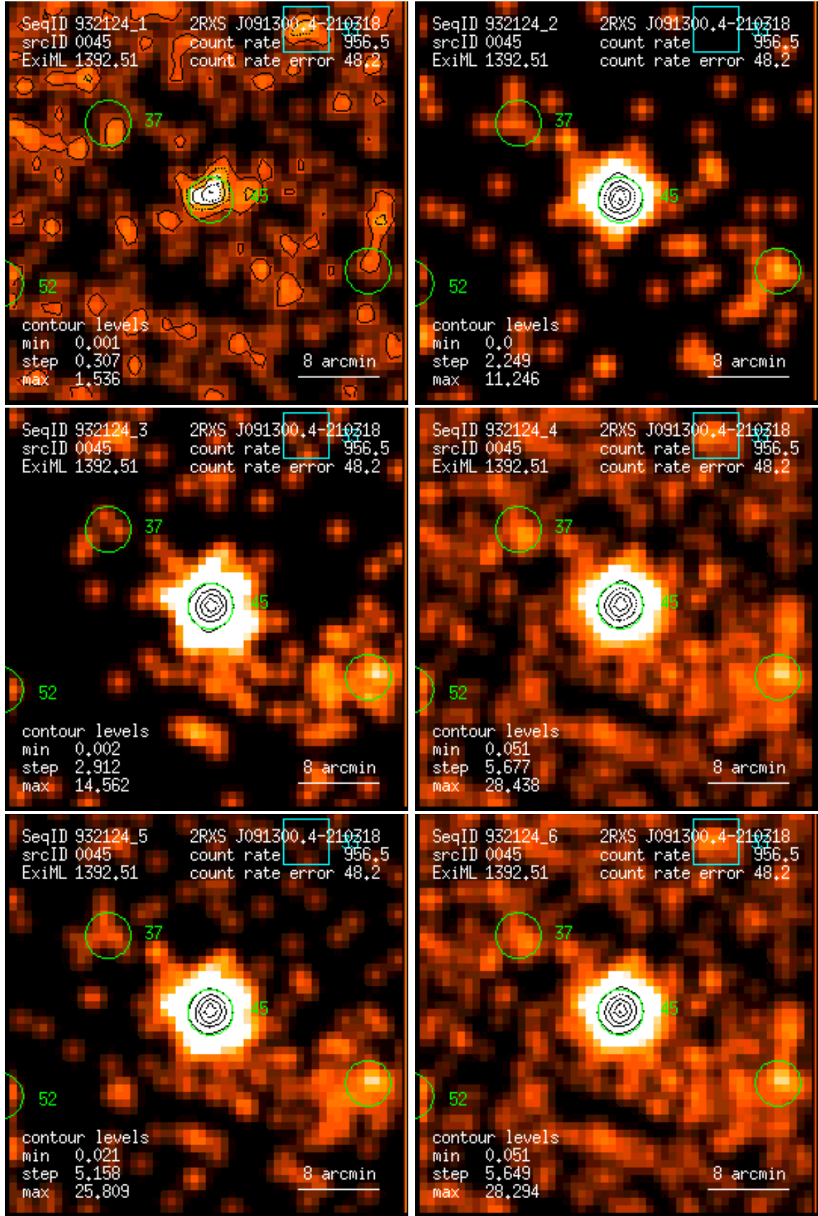
Figure 45: RASS 932124: detection 0045: band rate images, Gaussian filter: (1) PSPC channels 11 – 41, (2) 52 – 90, (3) 91 – 201, (4) 11 – 235, (5) 52 – 201, (6) 11 – 201. Broad band rates in counts/ks. Band rate contour levels in counts/ks/arcmin 2 .
