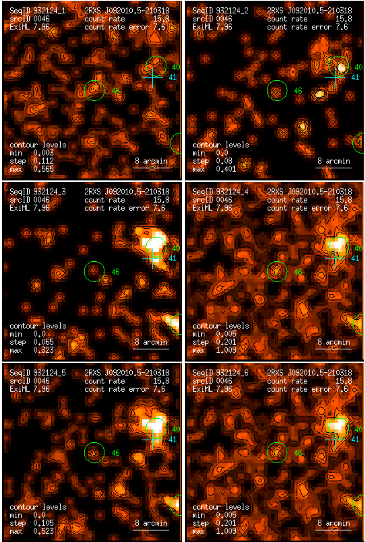
Figure 46: RASS 932124: detection 0046: band rate images, Gaussian filter: (1) PSPC channels 11 – 41, (2) 52 – 90, (3) 91 – 201, (4) 11 – 235, (5) 52 – 201, (6) 11 – 201. Broad band rates in counts/ks. Band rate contour levels in counts/ks/arcmin 2 .
