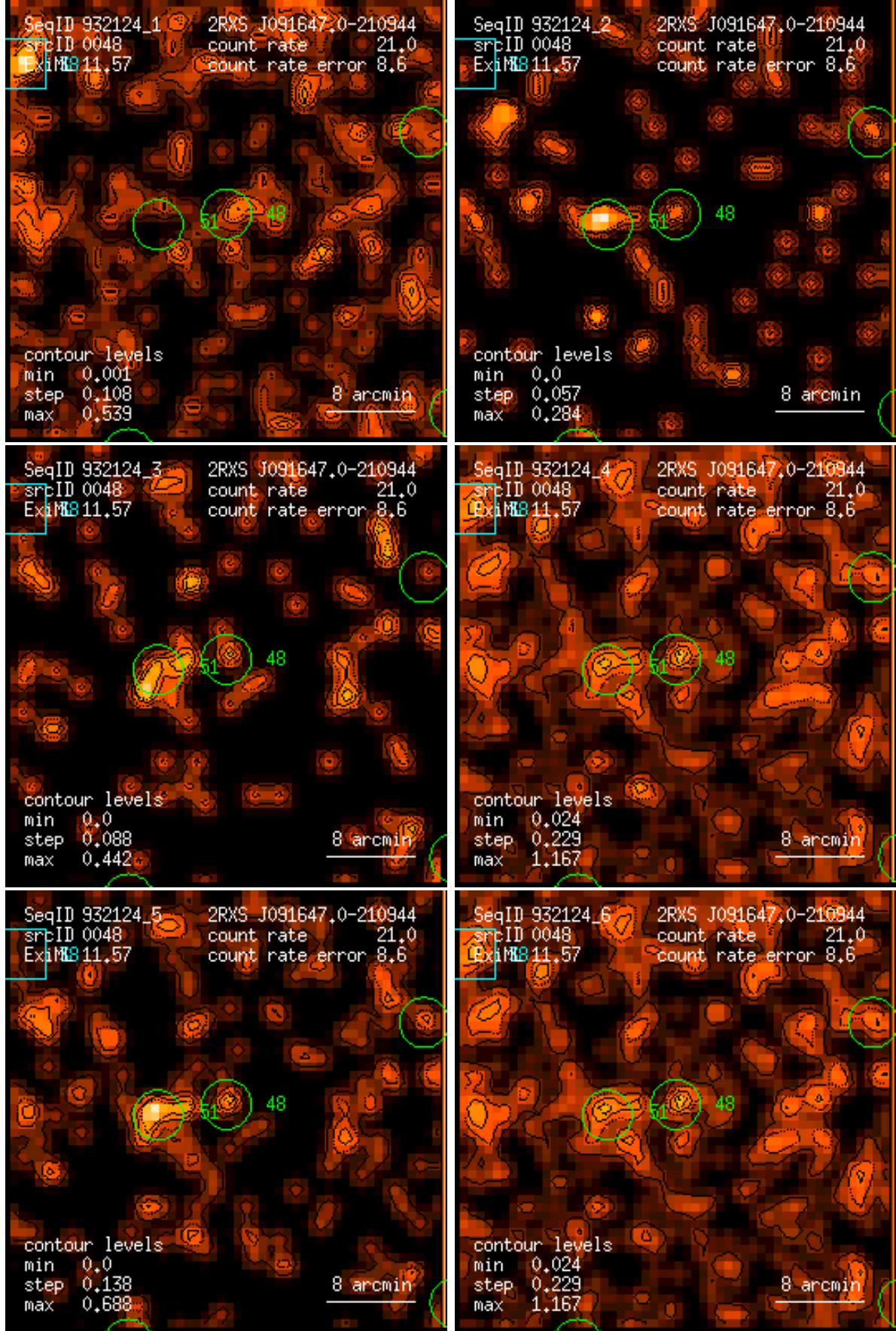
Figure 48: RASS 932124: detection 0048: band rate images, Gaussian filter: (1) PSPC channels 11 – 41, (2) 52 – 90, (3) 91 – 201, (4) 11 – 235, (5) 52 – 201, (6) 11 – 201. Broad band rates in counts/ks. Band rate contour levels in counts/ks/arcmin 2 .
