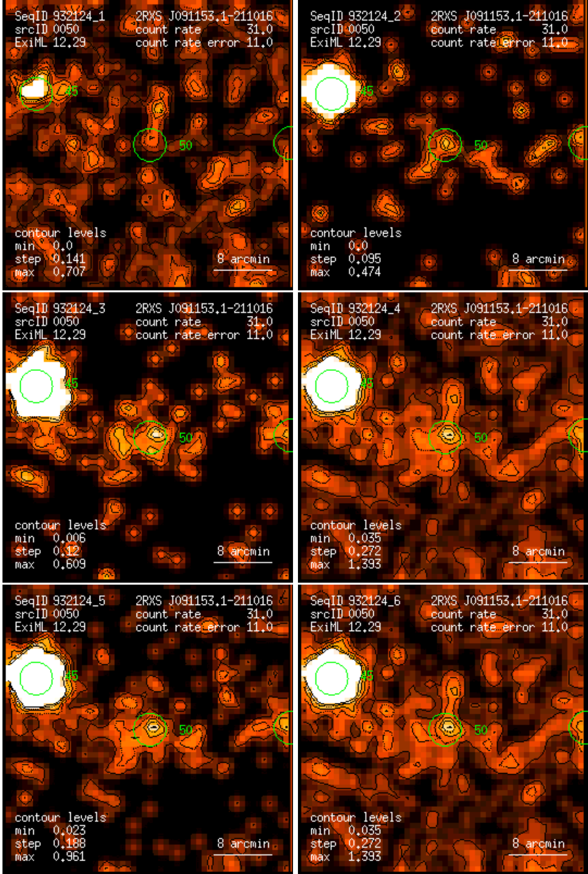
Figure 50: RASS 932124: detection 0050: band rate images, Gaussian filter: (1) PSPC channels 11 – 41, (2) 52 – 90, (3) 91 – 201, (4) 11 – 235, (5) 52 – 201, (6) 11 – 201. Broad band rates in counts/ks. Band rate contour levels in counts/ks/arcmin 2 .
