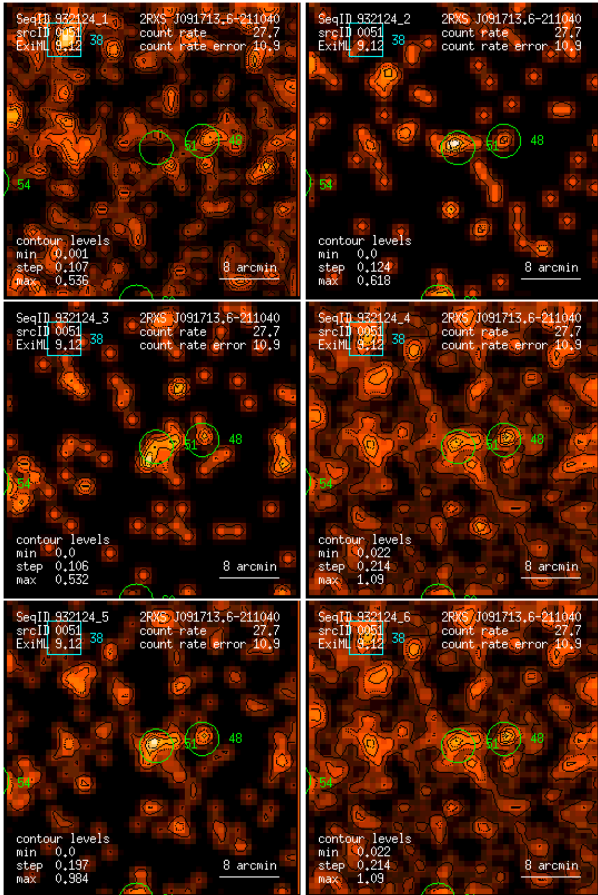
Figure 51: RASS 932124: detection 0051: band rate images, Gaussian filter: (1) PSPC channels 11 – 41, (2) 52 – 90, (3) 91 – 201, (4) 11 – 235, (5) 52 – 201, (6) 11 – 201. Broad band rates in counts/ks. Band rate contour levels in counts/ks/arcmin 2 .
