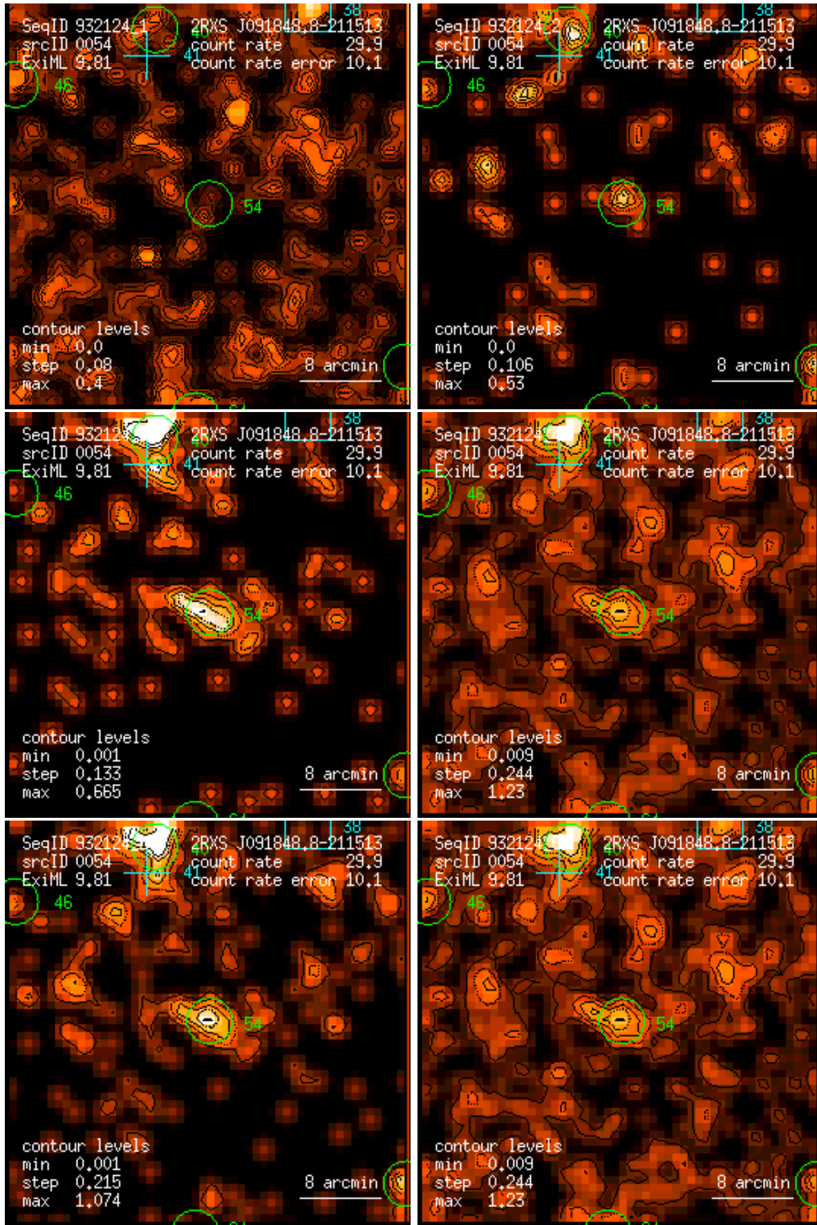
Figure 54: RASS 932124: detection 0054: band rate images, Gaussian filter: (1) PSPC channels 11 – 41, (2) 52 – 90, (3) 91 – 201, (4) 11 – 235, (5) 52 – 201, (6) 11 – 201. Broad band rates in counts/ks. Band rate contour levels in counts/ks/arcmin 2 .
