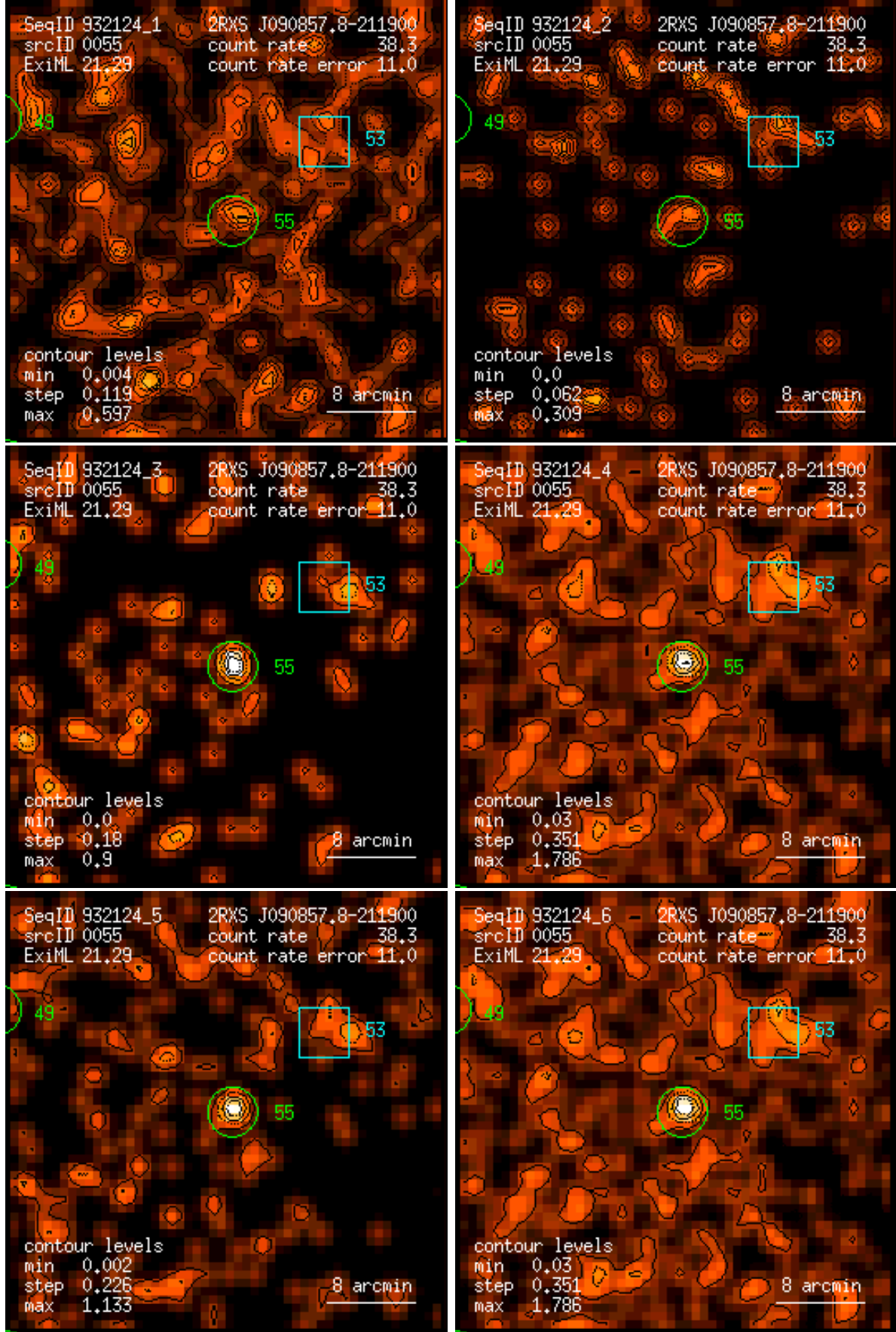
Figure 55: RASS 932124: detection 0055: band rate images, Gaussian filter: (1) PSPC channels 11 – 41, (2) 52 – 90, (3) 91 – 201, (4) 11 – 235, (5) 52 – 201, (6) 11 – 201. Broad band rates in counts/ks. Band rate contour levels in counts/ks/arcmin 2 .
