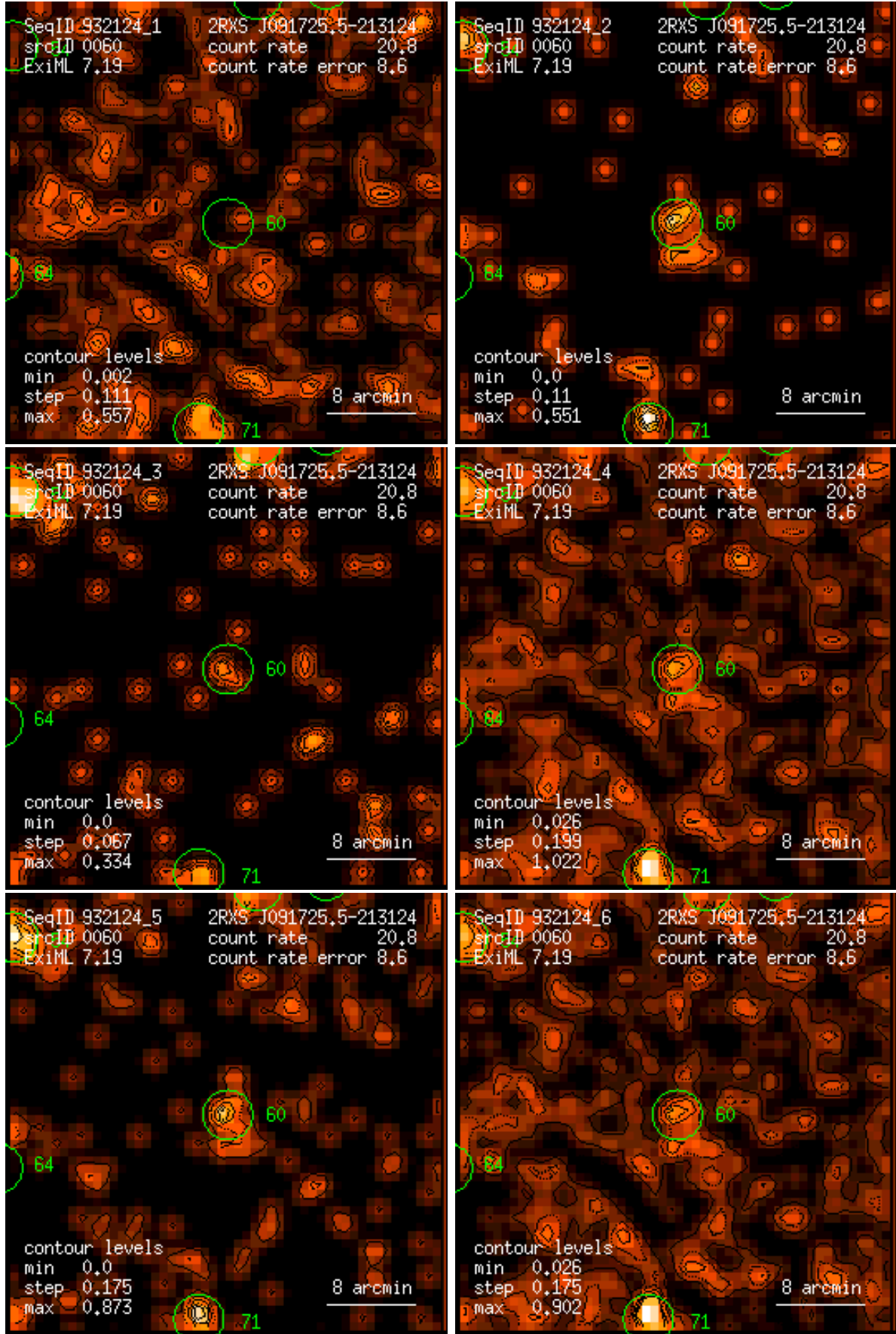
Figure 60: RASS 932124: detection 0060: band rate images, Gaussian filter: (1) PSPC channels 11 – 41, (2) 52 – 90, (3) 91 – 201, (4) 11 – 235, (5) 52 – 201, (6) 11 – 201. Broad band rates in counts/ks. Band rate contour levels in counts/ks/arcmin 2 .
