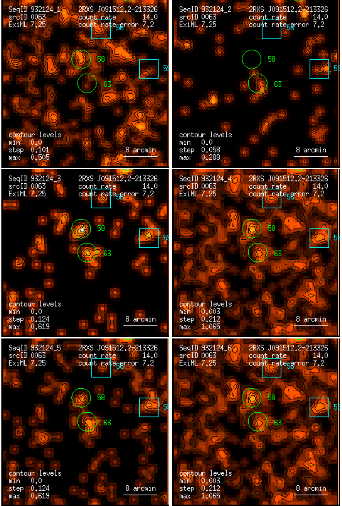
Figure 63: RASS 932124: detection 0063: band rate images, Gaussian filter: (1) PSPC channels 11 – 41, (2) 52 – 90, (3) 91 – 201, (4) 11 – 235, (5) 52 – 201, (6) 11 – 201. Broad band rates in counts/ks. Band rate contour levels in counts/ks/arcmin 2 .
