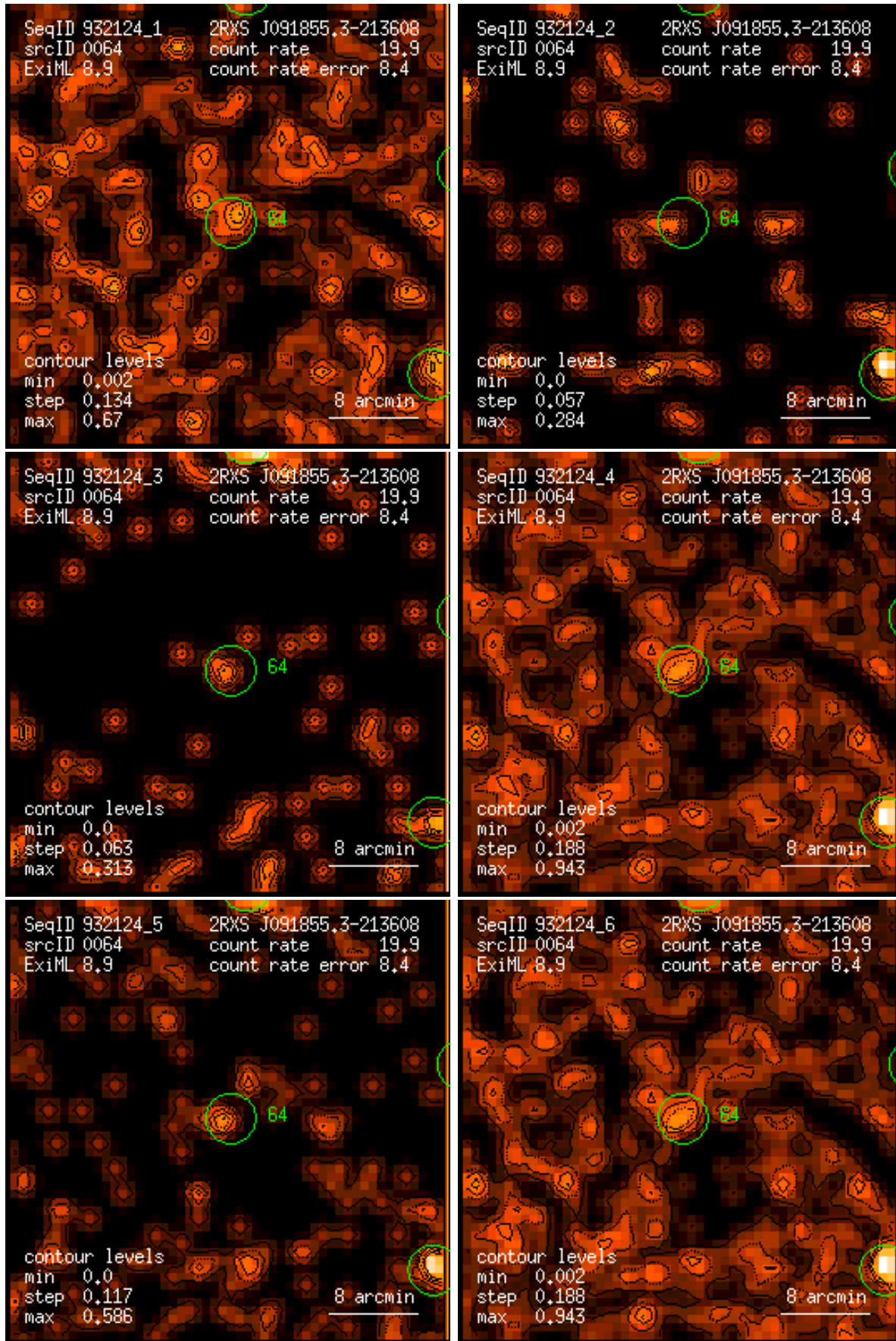
Figure 64: RASS 932124: detection 0064: band rate images, Gaussian filter: (1) PSPC channels 11 – 41, (2) 52 – 90, (3) 91 – 201, (4) 11 – 235, (5) 52 – 201, (6) 11 – 201. Broad band rates in counts/ks. Band rate contour levels in counts/ks/arcmin 2 .
