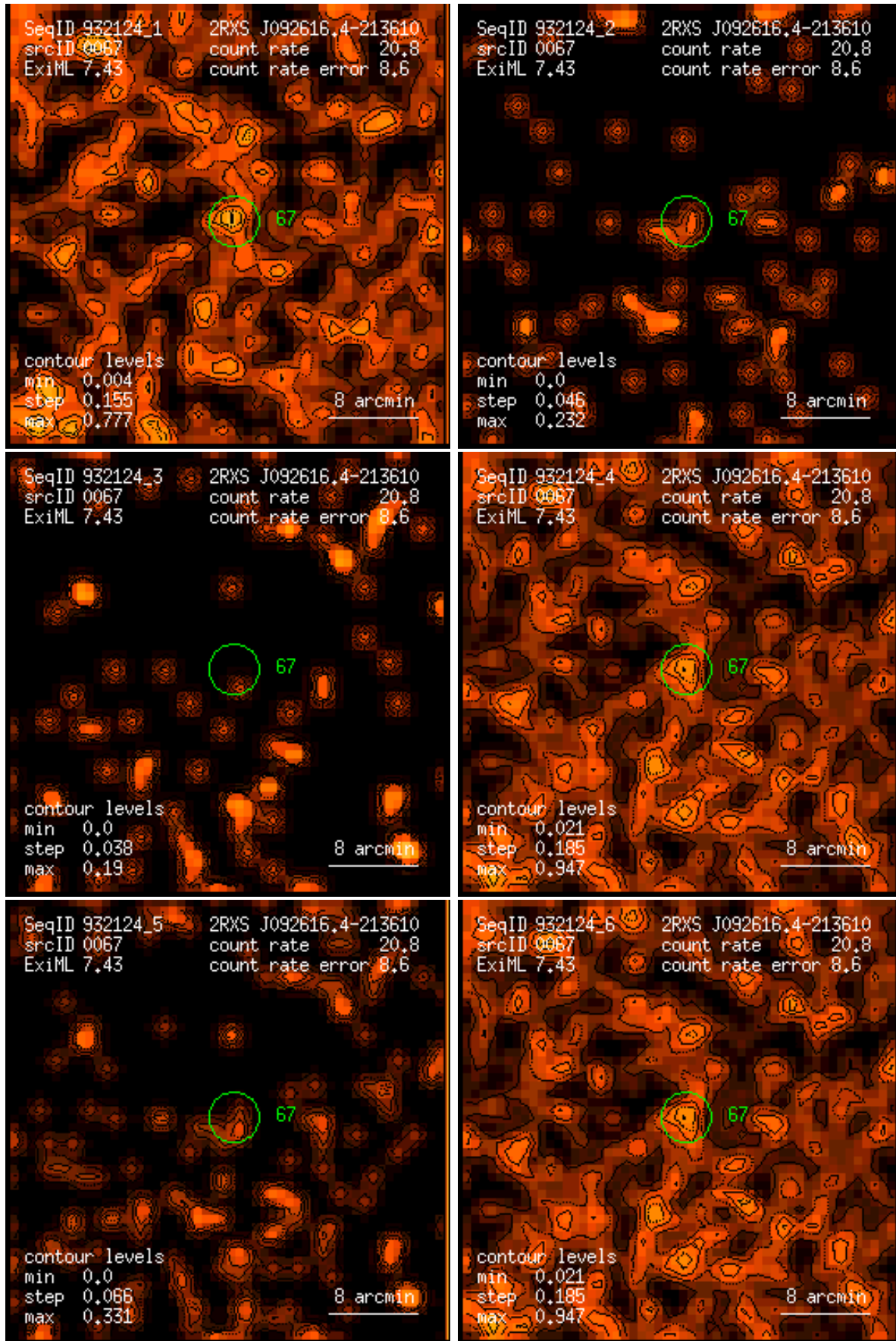
Figure 67: RASS 932124: detection 0067: band rate images, Gaussian filter: (1) PSPC channels 11 – 41, (2) 52 – 90, (3) 91 – 201, (4) 11 – 235, (5) 52 – 201, (6) 11 – 201. Broad band rates in counts/ks. Band rate contour levels in counts/ks/arcmin 2 .
