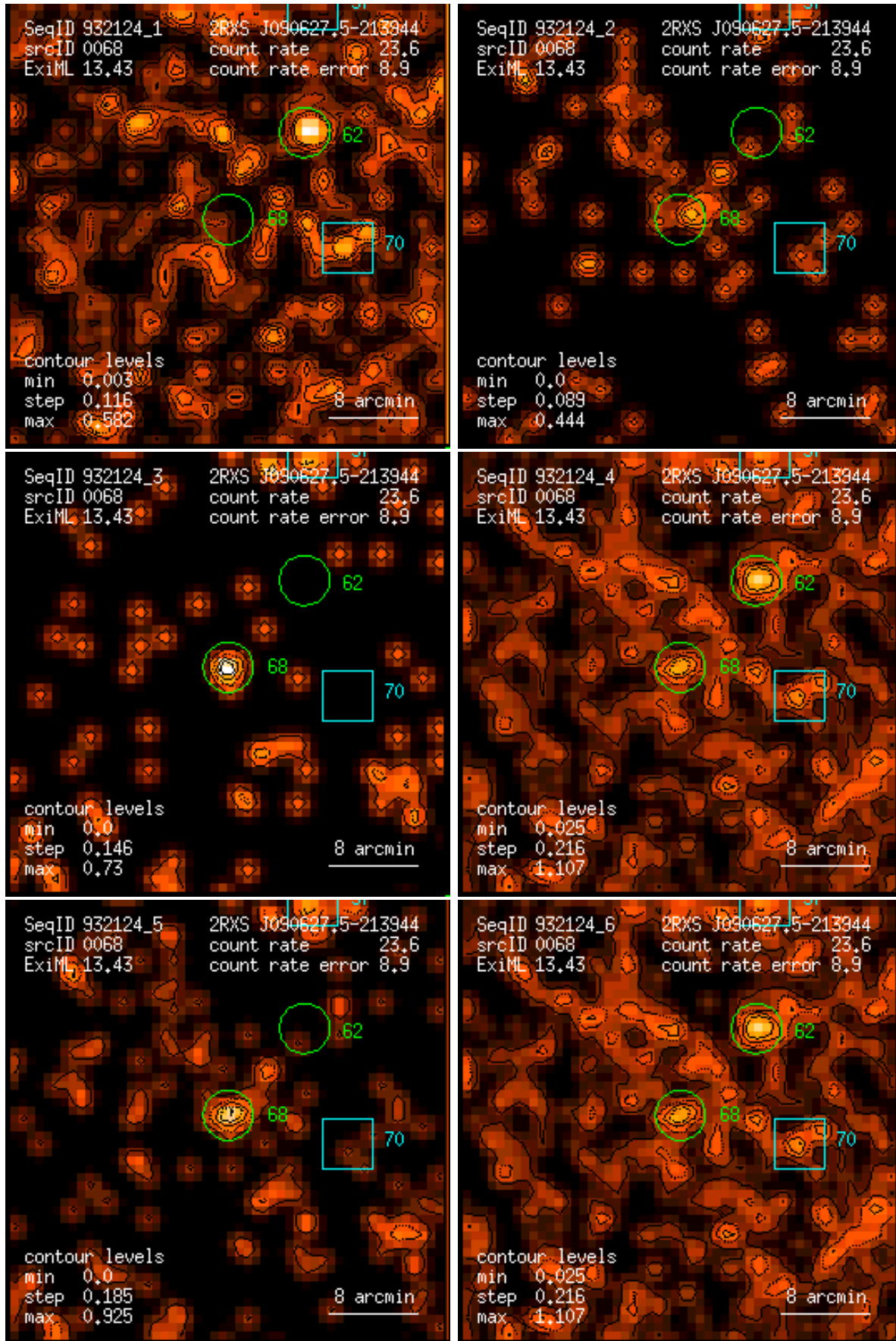
Figure 68: RASS 932124: detection 0068: band rate images, Gaussian filter: (1) PSPC channels 11 – 41, (2) 52 – 90, (3) 91 – 201, (4) 11 – 235, (5) 52 – 201, (6) 11 – 201. Broad band rates in counts/ks. Band rate contour levels in counts/ks/arcmin 2 .
