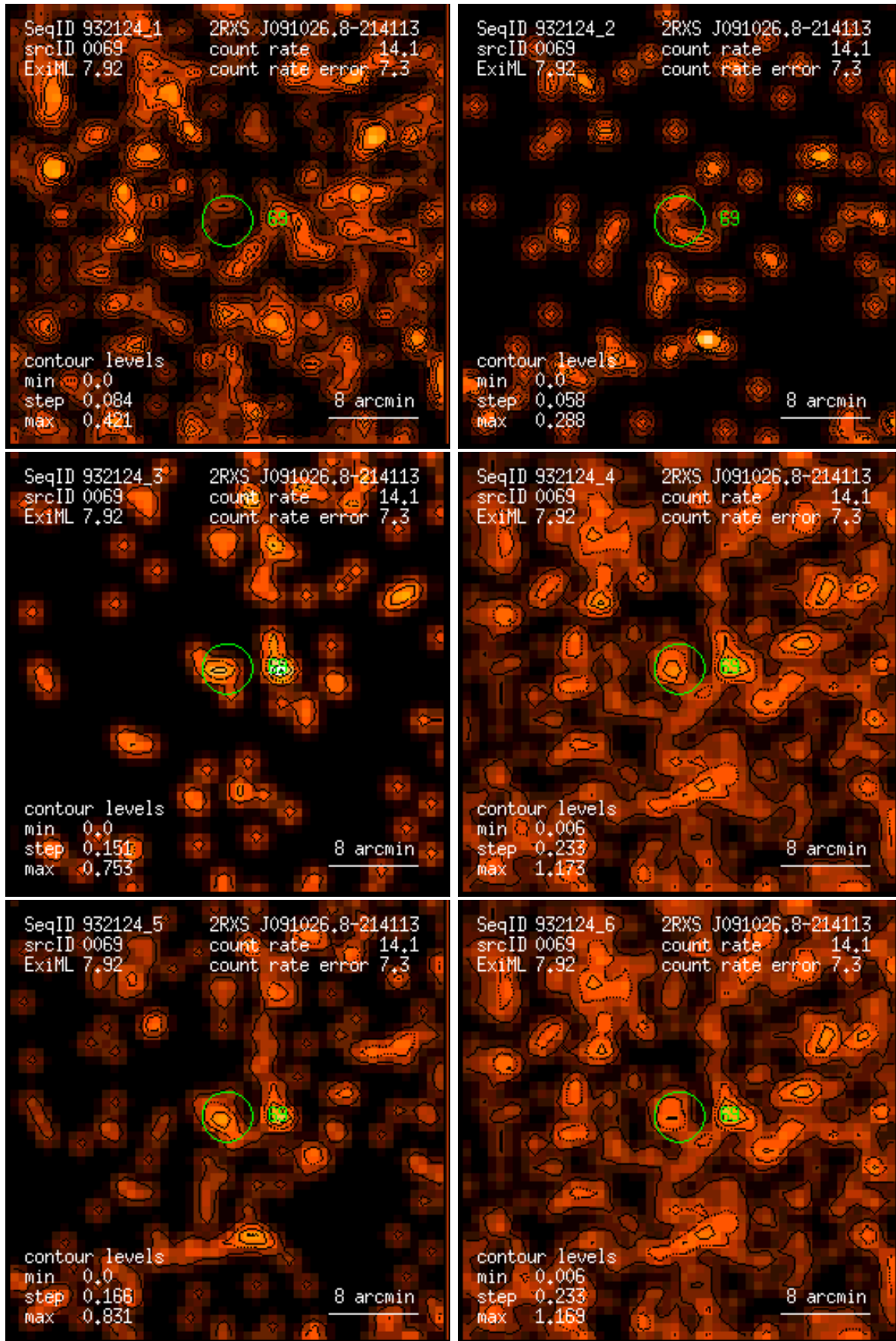
Figure 69: RASS 932124: detection 0069: band rate images, Gaussian filter: (1) PSPC channels 11 – 41, (2) 52 – 90, (3) 91 – 201, (4) 11 – 235, (5) 52 – 201, (6) 11 – 201. Broad band rates in counts/ks. Band rate contour levels in counts/ks/arcmin 2 .
