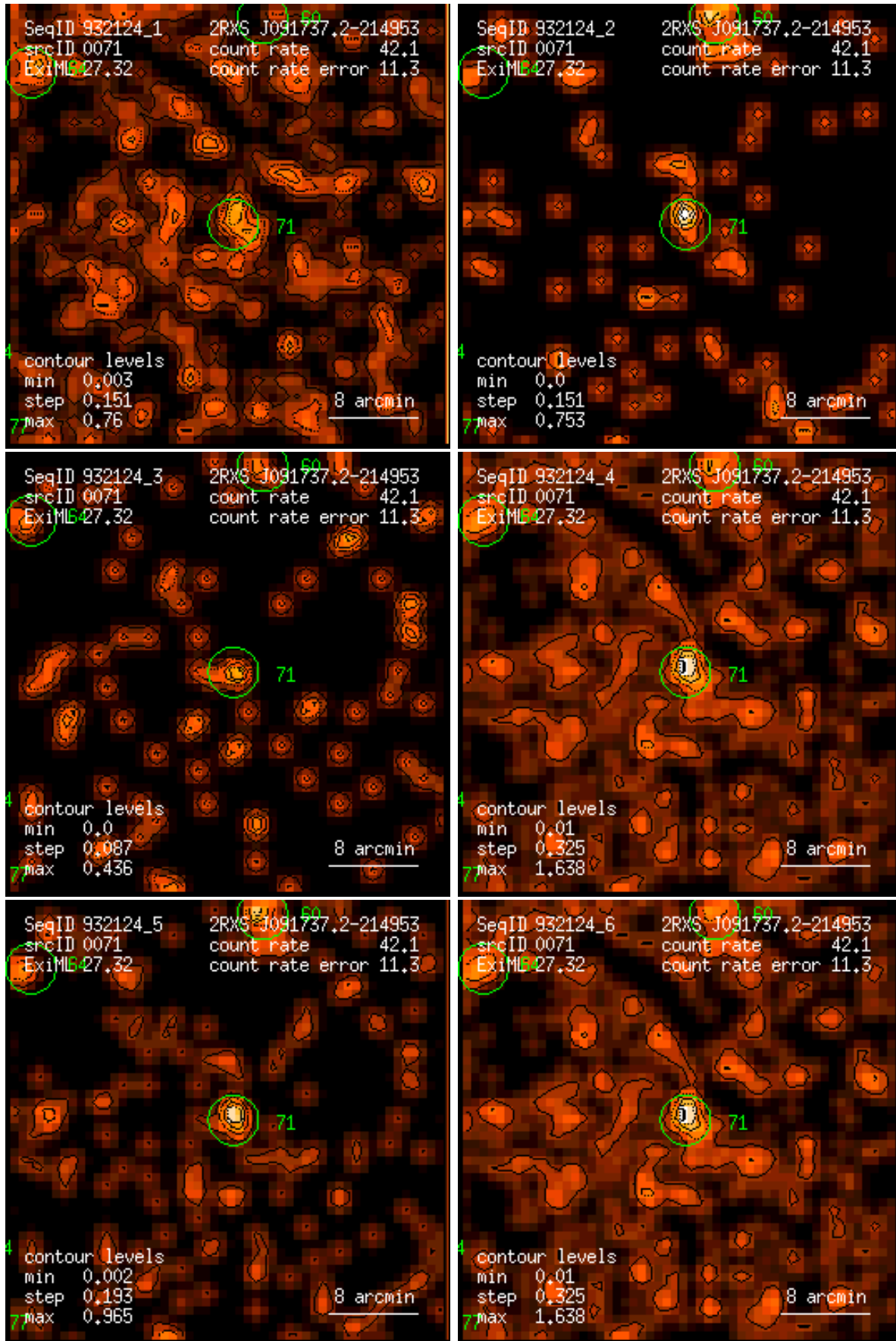
Figure 71: RASS 932124: detection 0071: band rate images, Gaussian filter: (1) PSPC channels 11 – 41, (2) 52 – 90, (3) 91 – 201, (4) 11 – 235, (5) 52 – 201, (6) 11 – 201. Broad band rates in counts/ks. Band rate contour levels in counts/ks/arcmin 2 .
