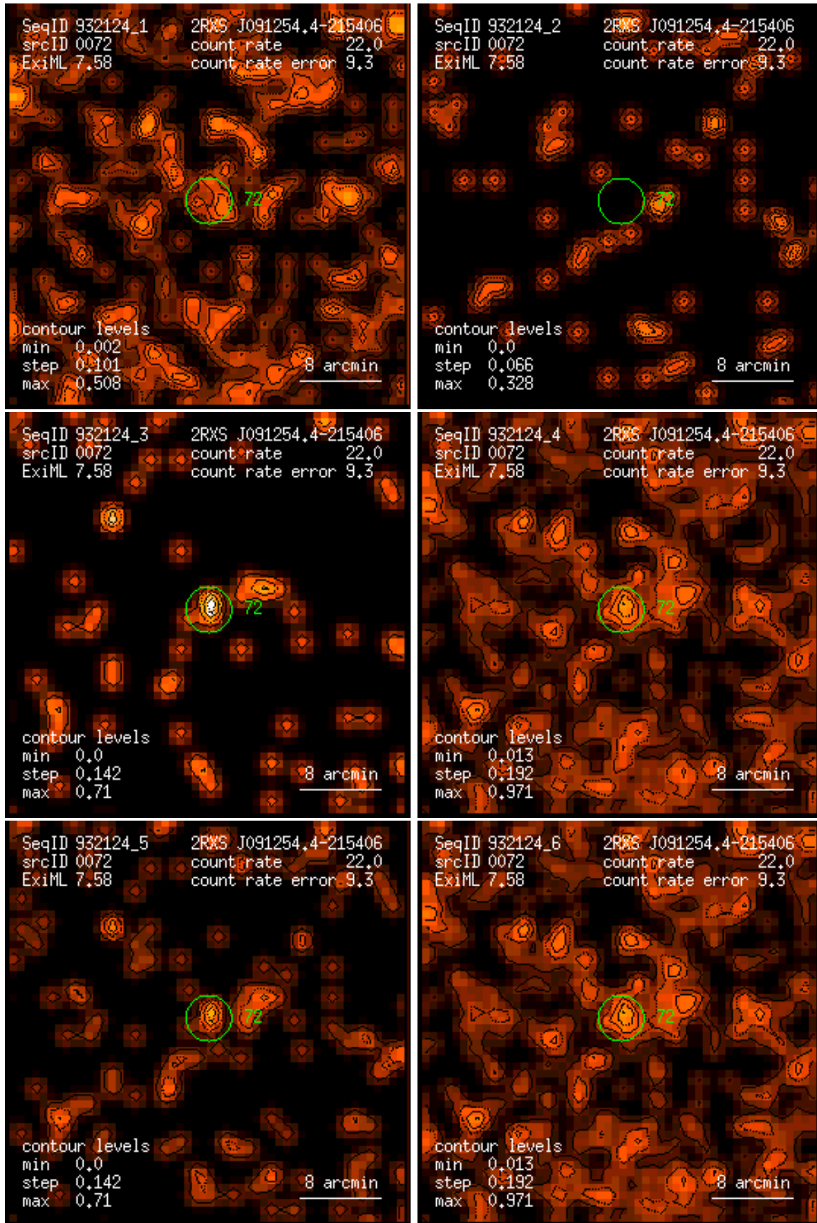
Figure 72: RASS 932124: detection 0072: band rate images, Gaussian filter: (1) PSPC channels 11 – 41, (2) 52 – 90, (3) 91 – 201, (4) 11 – 235, (5) 52 – 201, (6) 11 – 201. Broad band rates in counts/ks. Band rate contour levels in counts/ks/arcmin 2 .
