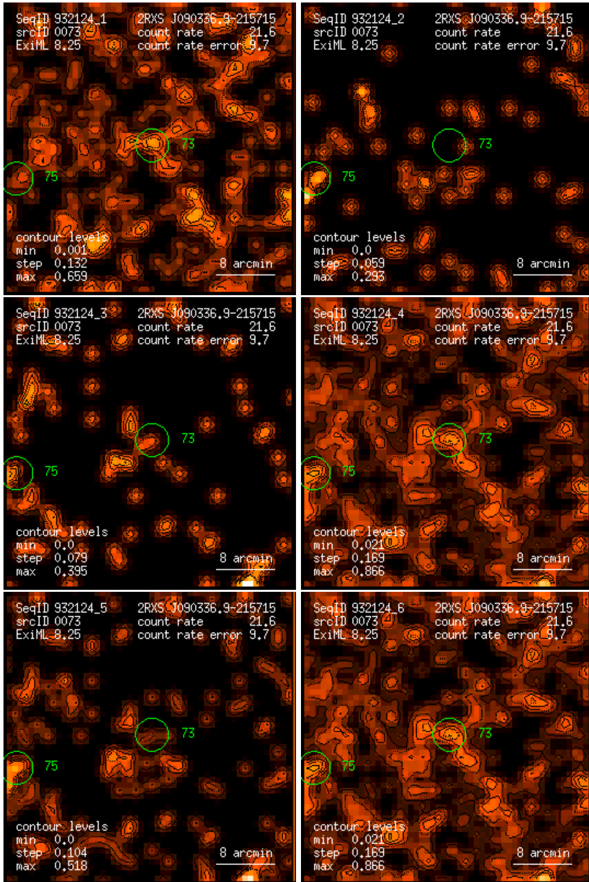
Figure 73: RASS 932124: detection 0073: band rate images, Gaussian filter: (1) PSPC channels 11 – 41, (2) 52 – 90, (3) 91 – 201, (4) 11 – 235, (5) 52 – 201, (6) 11 – 201. Broad band rates in counts/ks. Band rate contour levels in counts/ks/arcmin 2 .
