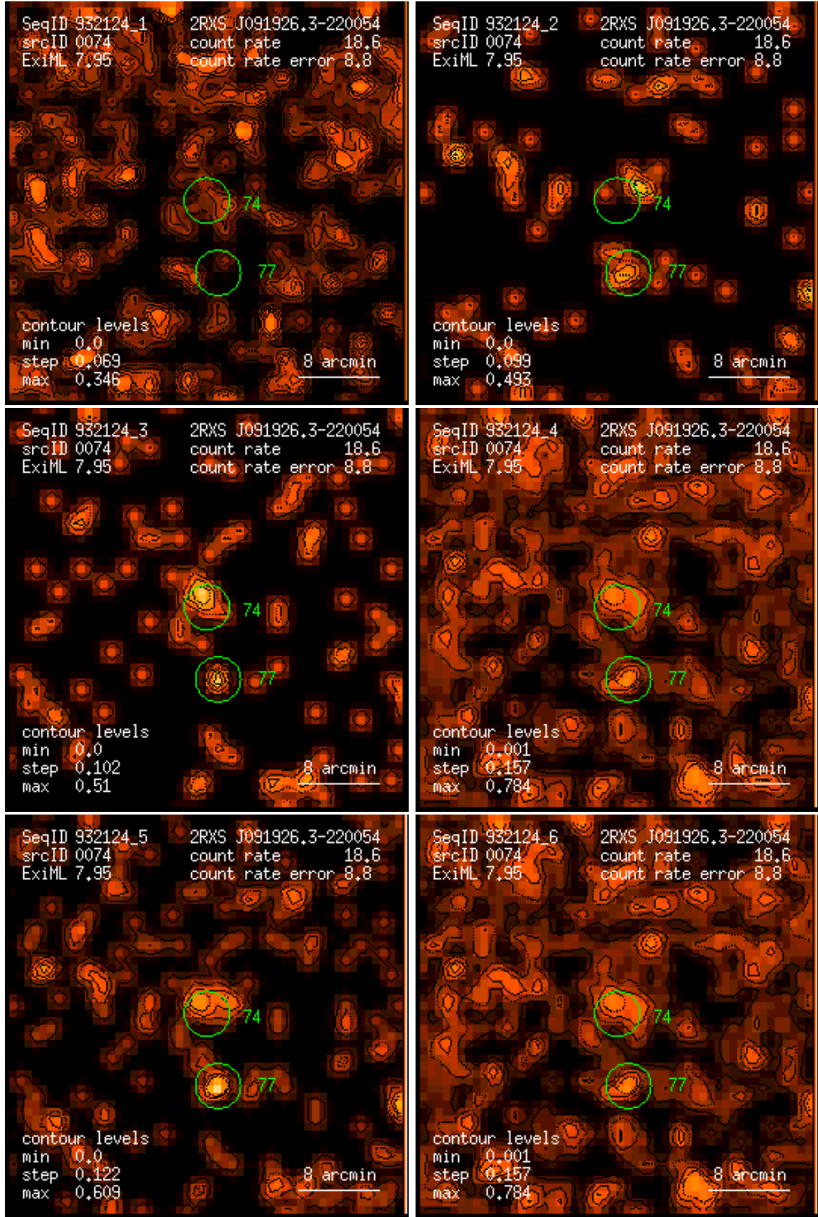
Figure 74: RASS 932124: detection 0074: band rate images, Gaussian filter: (1) PSPC channels 11 – 41, (2) 52 – 90, (3) 91 – 201, (4) 11 – 235, (5) 52 – 201, (6) 11 – 201. Broad band rates in counts/ks. Band rate contour levels in counts/ks/arcmin 2 .
