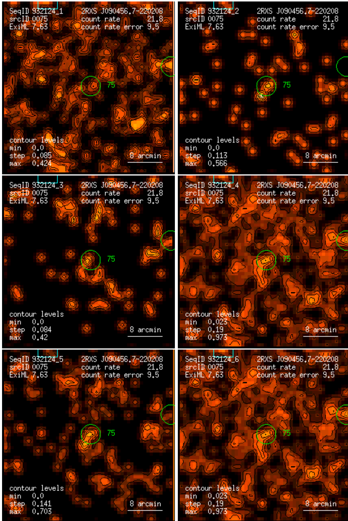
Figure 75: RASS 932124: detection 0075: band rate images, Gaussian filter: (1) PSPC channels 11 – 41, (2) 52 – 90, (3) 91 – 201, (4) 11 – 235, (5) 52 – 201, (6) 11 – 201. Broad band rates in counts/ks. Band rate contour levels in counts/ks/arcmin 2 .
