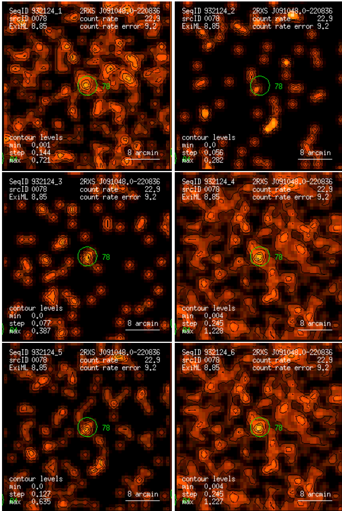
Figure 78: RASS 932124: detection 0078: band rate images, Gaussian filter: (1) PSPC channels 11 – 41, (2) 52 – 90, (3) 91 – 201, (4) 11 – 235, (5) 52 – 201, (6) 11 – 201. Broad band rates in counts/ks. Band rate contour levels in counts/ks/arcmin 2 .
