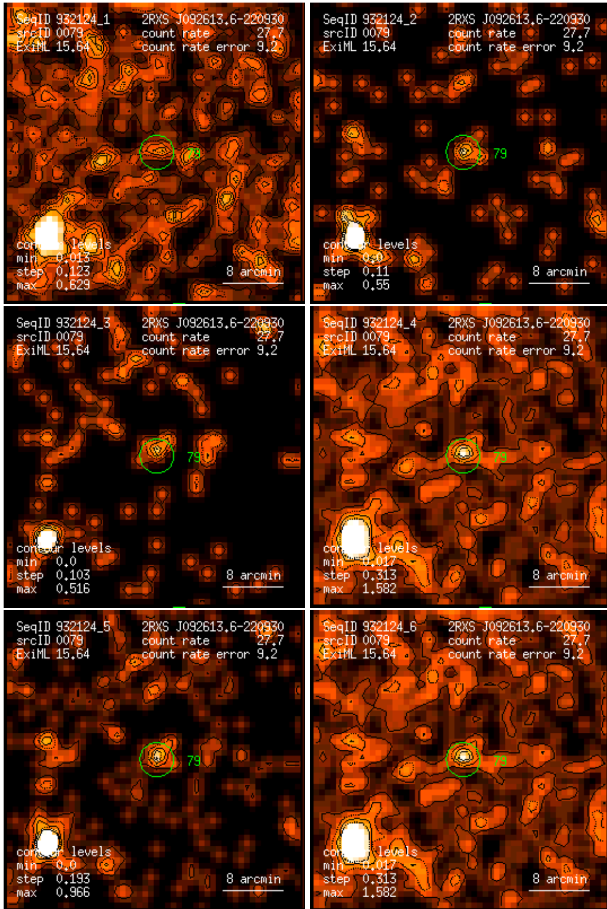
Figure 79: RASS 932124: detection 0079: band rate images, Gaussian filter: (1) PSPC channels 11 – 41, (2) 52 – 90, (3) 91 – 201, (4) 11 – 235, (5) 52 – 201, (6) 11 – 201. Broad band rates in counts/ks. Band rate contour levels in counts/ks/arcmin 2 .
