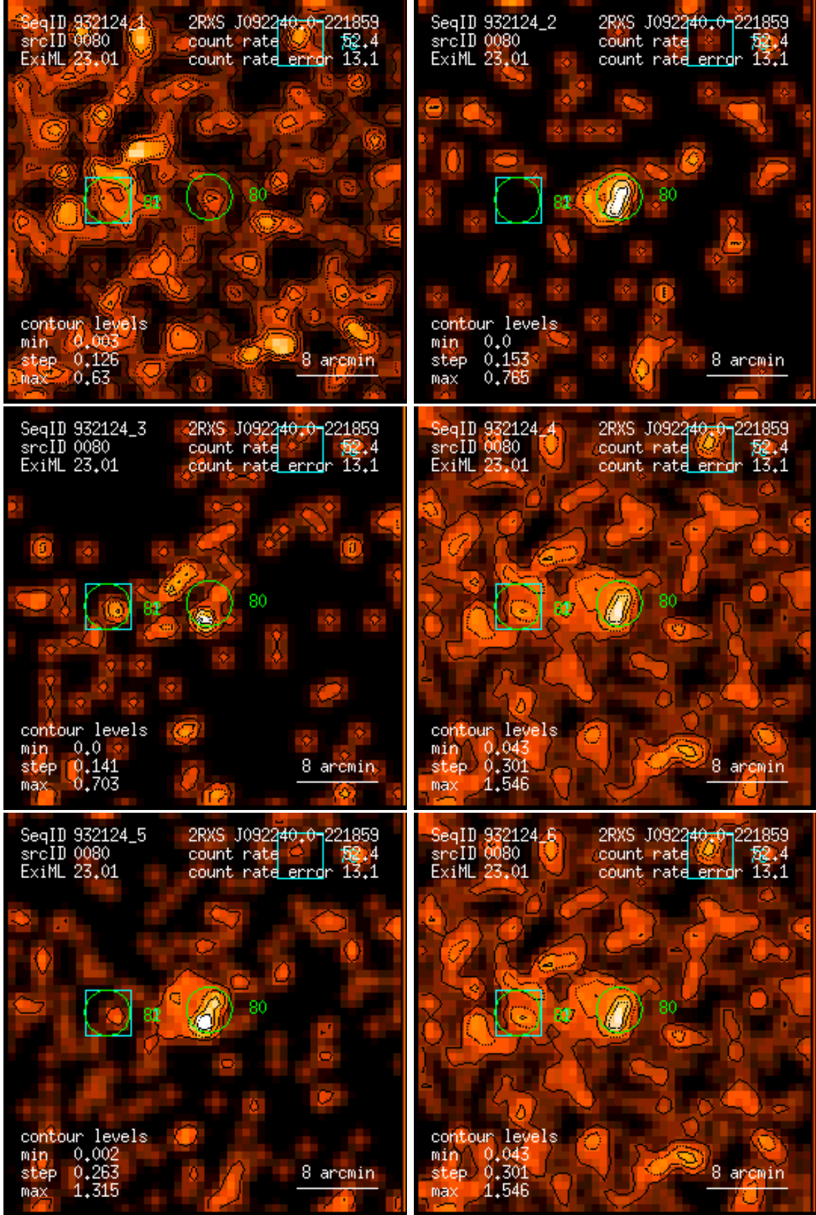
Figure 80: RASS 932124: detection 0080: band rate images, Gaussian filter: (1) PSPC channels 11 – 41, (2) 52 – 90, (3) 91 – 201, (4) 11 – 235, (5) 52 – 201, (6) 11 – 201. Broad band rates in counts/ks. Band rate contour levels in counts/ks/arcmin 2 .
