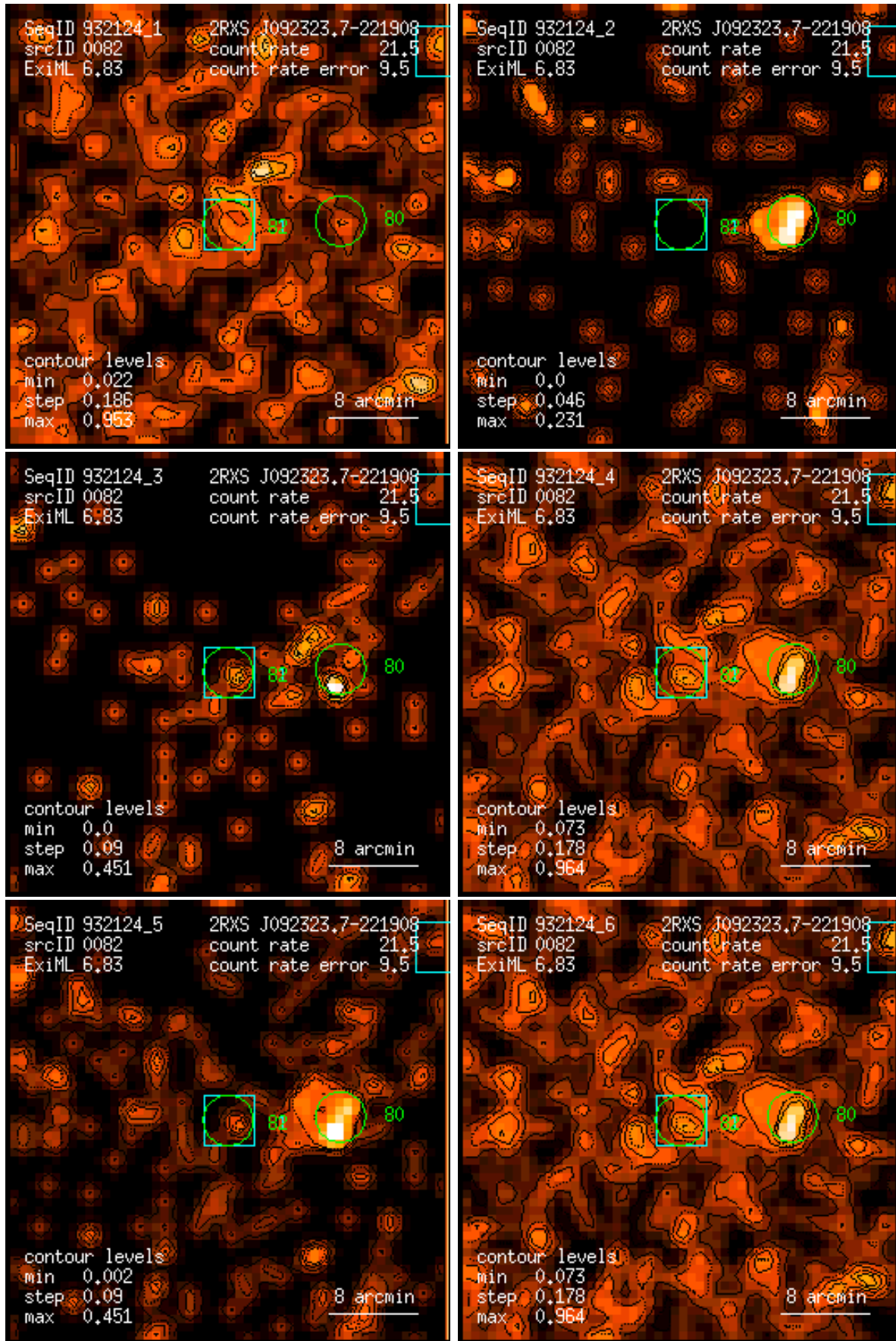
Figure 82: RASS 932124: detection 0082: band rate images, Gaussian filter: (1) PSPC channels 11 – 41, (2) 52 – 90, (3) 91 – 201, (4) 11 – 235, (5) 52 – 201, (6) 11 – 201. Broad band rates in counts/ks. Band rate contour levels in counts/ks/arcmin 2 .
