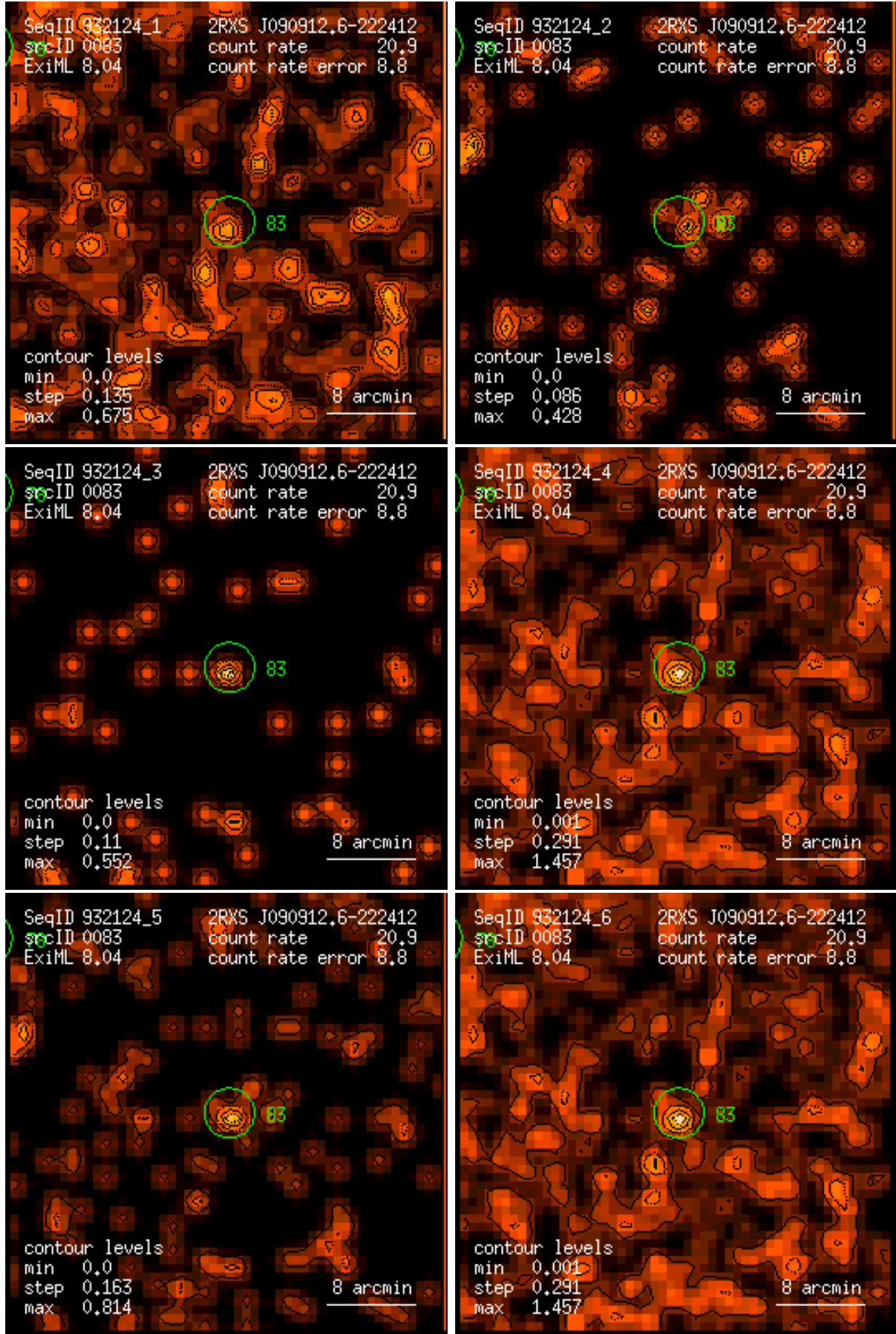
Figure 83: RASS 932124: detection 0083: band rate images, Gaussian filter: (1) PSPC channels 11 – 41, (2) 52 – 90, (3) 91 – 201, (4) 11 – 235, (5) 52 – 201, (6) 11 – 201. Broad band rates in counts/ks. Band rate contour levels in counts/ks/arcmin 2 .
